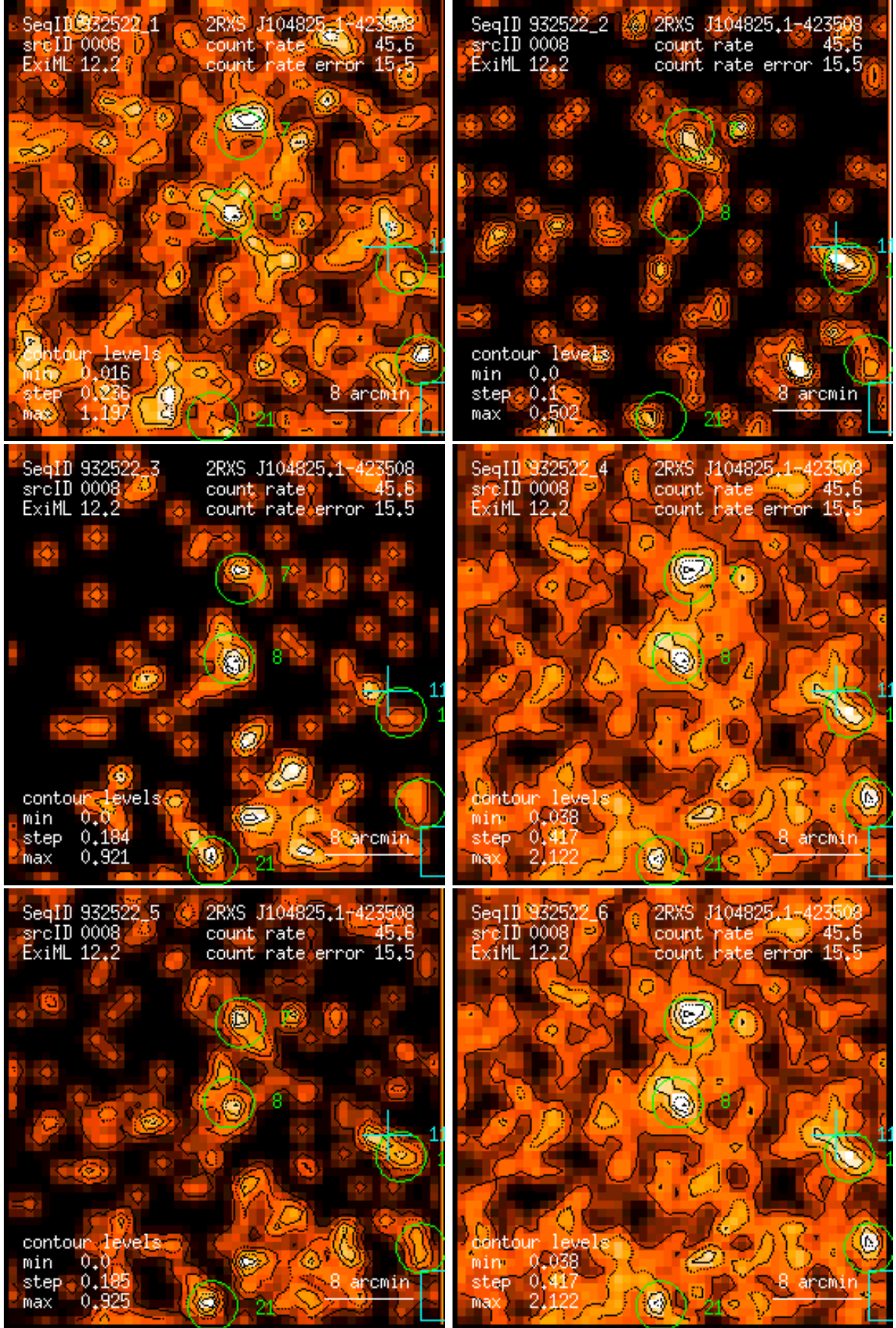
Figure 8: RASS 932522: detection 0008: band rate images, Gaussian filter: (1) PSPC channels 11 – 41, (2) 52 – 90, (3) 91 – 201, (4) 11 – 235, (5) 52 – 201, (6) 11 – 201. Broad band rates in counts/ks. Band rate contour levels in counts/ks/arcmin 2 .
