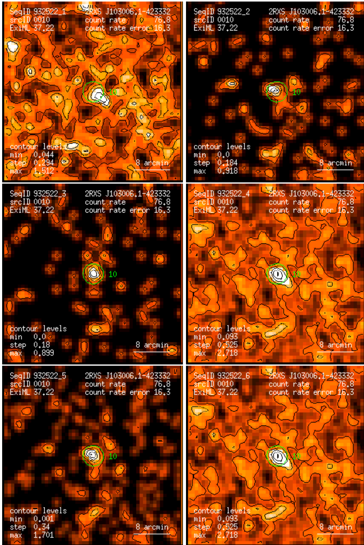
Figure 10: RASS 932522: detection 0010: band rate images, Gaussian filter: (1) PSPC channels 11 – 41, (2) 52 – 90, (3) 91 – 201, (4) 11 – 235, (5) 52 – 201, (6) 11 – 201. Broad band rates in counts/ks. Band rate contour levels in counts/ks/arcmin 2 .
