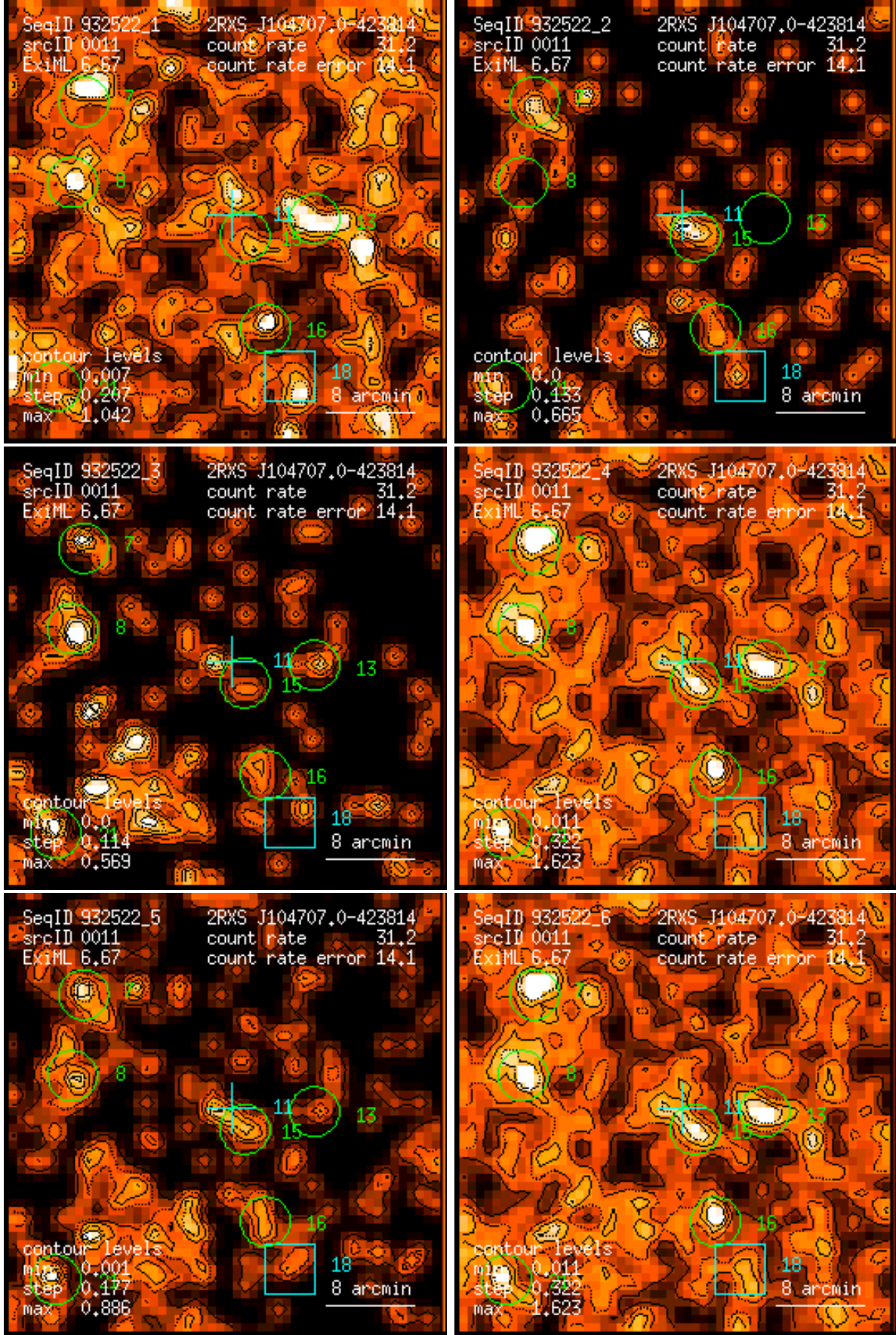
Figure 11: RASS 932522: detection 0011: band rate images, Gaussian filter: (1) PSPC channels 11 – 41, (2) 52 – 90, (3) 91 – 201, (4) 11 – 235, (5) 52 – 201, (6) 11 – 201. Broad band rates in counts/ks. Band rate contour levels in counts/ks/arcmin 2 .
