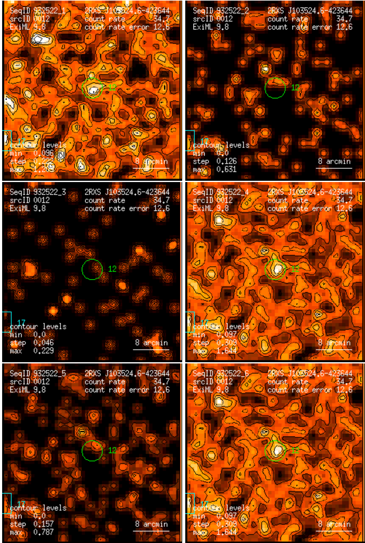
Figure 12: RASS 932522: detection 0012: band rate images, Gaussian filter: (1) PSPC channels 11 – 41, (2) 52 – 90, (3) 91 – 201, (4) 11 – 235, (5) 52 – 201, (6) 11 – 201. Broad band rates in counts/ks. Band rate contour levels in counts/ks/arcmin 2 .
