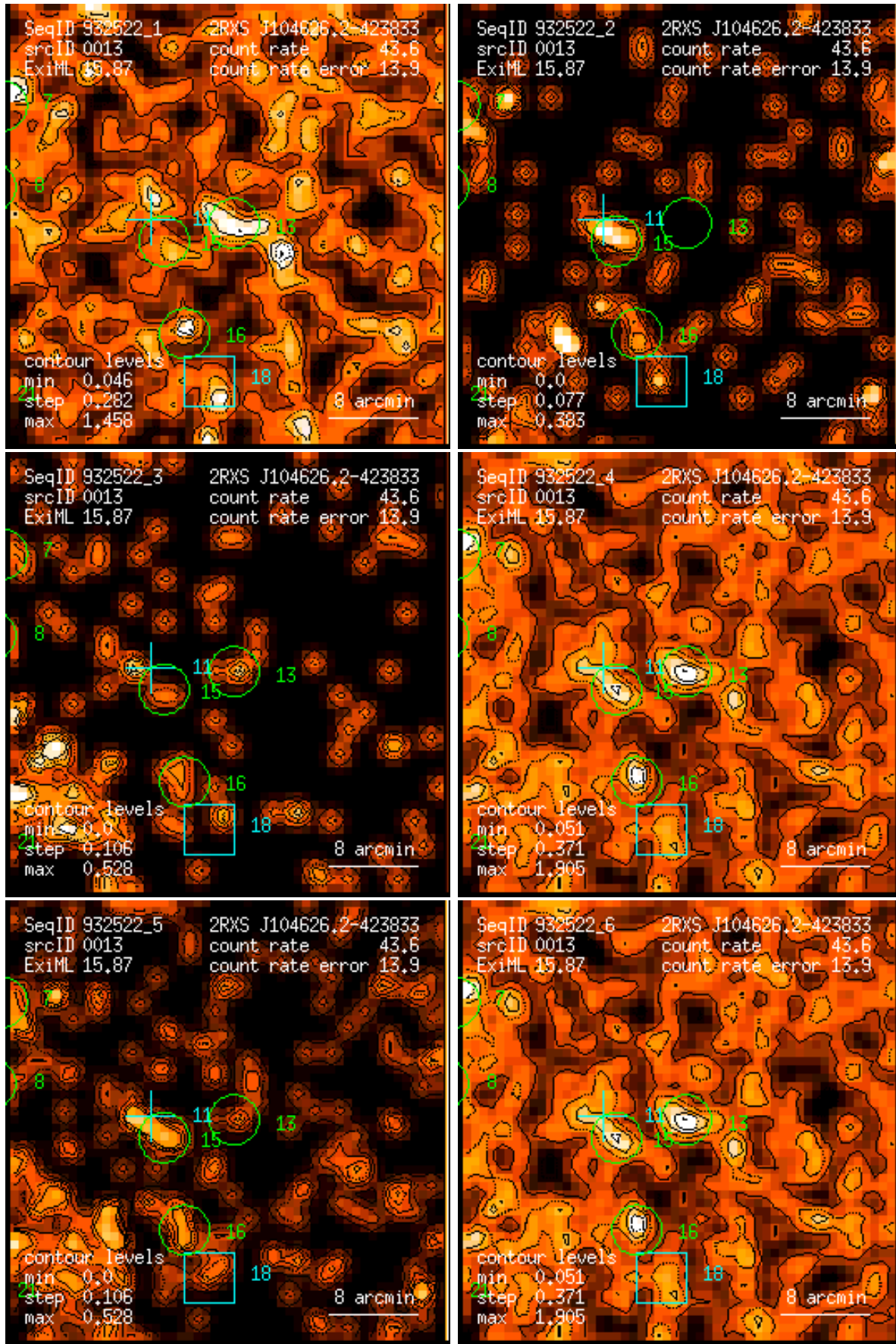
Figure 13: RASS 932522: detection 0013: band rate images, Gaussian filter: (1) PSPC channels 11 – 41, (2) 52 – 90, (3) 91 – 201, (4) 11 – 235, (5) 52 – 201, (6) 11 – 201. Broad band rates in counts/ks. Band rate contour levels in counts/ks/arcmin 2 .
