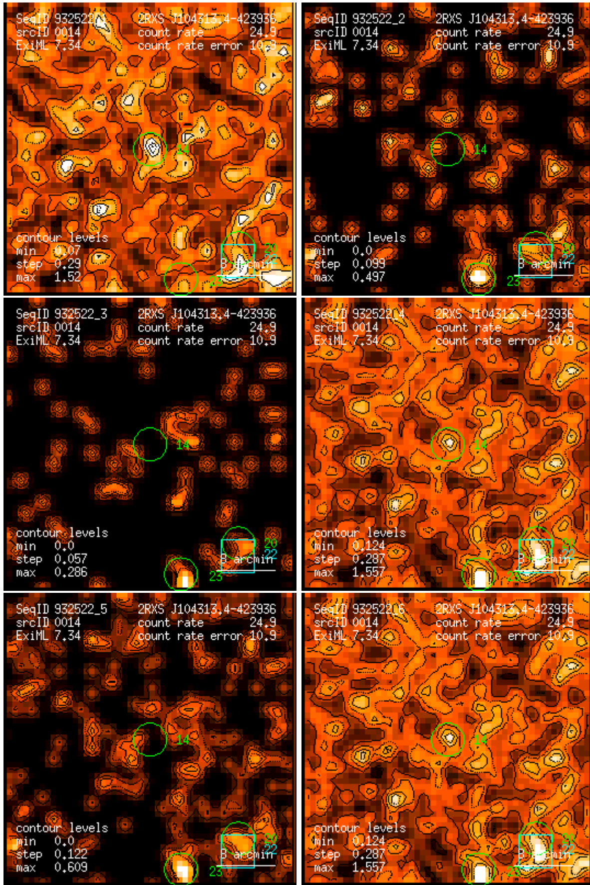
Figure 14: RASS 932522: detection 0014: band rate images, Gaussian filter: (1) PSPC channels 11 – 41, (2) 52 – 90, (3) 91 – 201, (4) 11 – 235, (5) 52 – 201, (6) 11 – 201. Broad band rates in counts/ks. Band rate contour levels in counts/ks/arcmin 2 .
