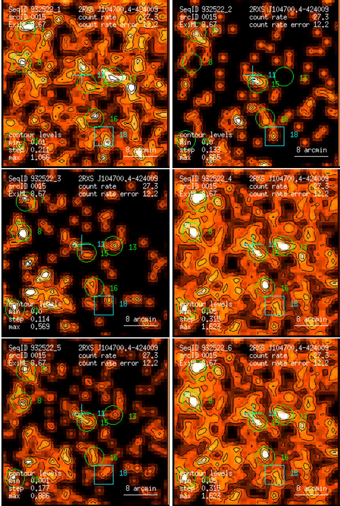
Figure 15: RASS 932522: detection 0015: band rate images, Gaussian filter: (1) PSPC channels 11 – 41, (2) 52 – 90, (3) 91 – 201, (4) 11 – 235, (5) 52 – 201, (6) 11 – 201. Broad band rates in counts/ks. Band rate contour levels in counts/ks/arcmin 2 .
