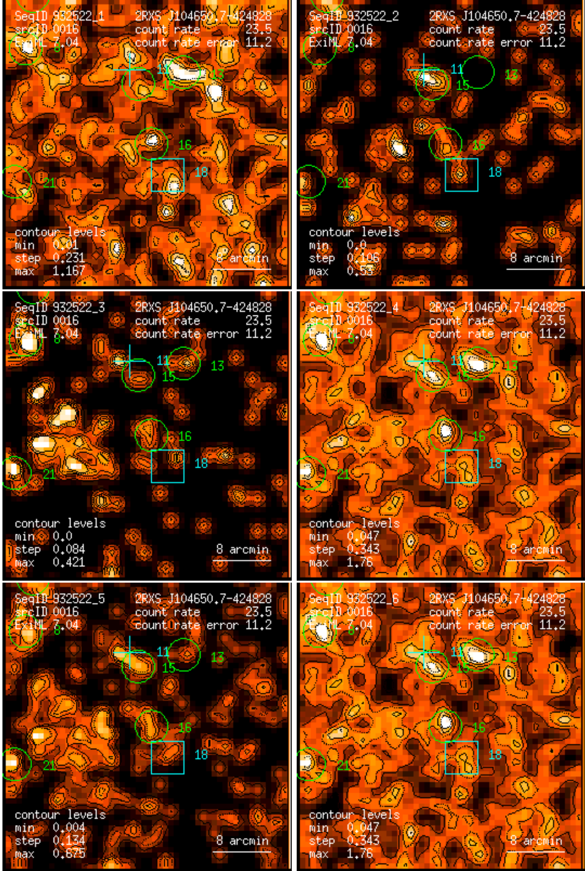
Figure 16: RASS 932522: detection 0016: band rate images, Gaussian filter: (1) PSPC channels 11 – 41, (2) 52 – 90, (3) 91 – 201, (4) 11 – 235, (5) 52 – 201, (6) 11 – 201. Broad band rates in counts/ks. Band rate contour levels in counts/ks/arcmin 2 .
