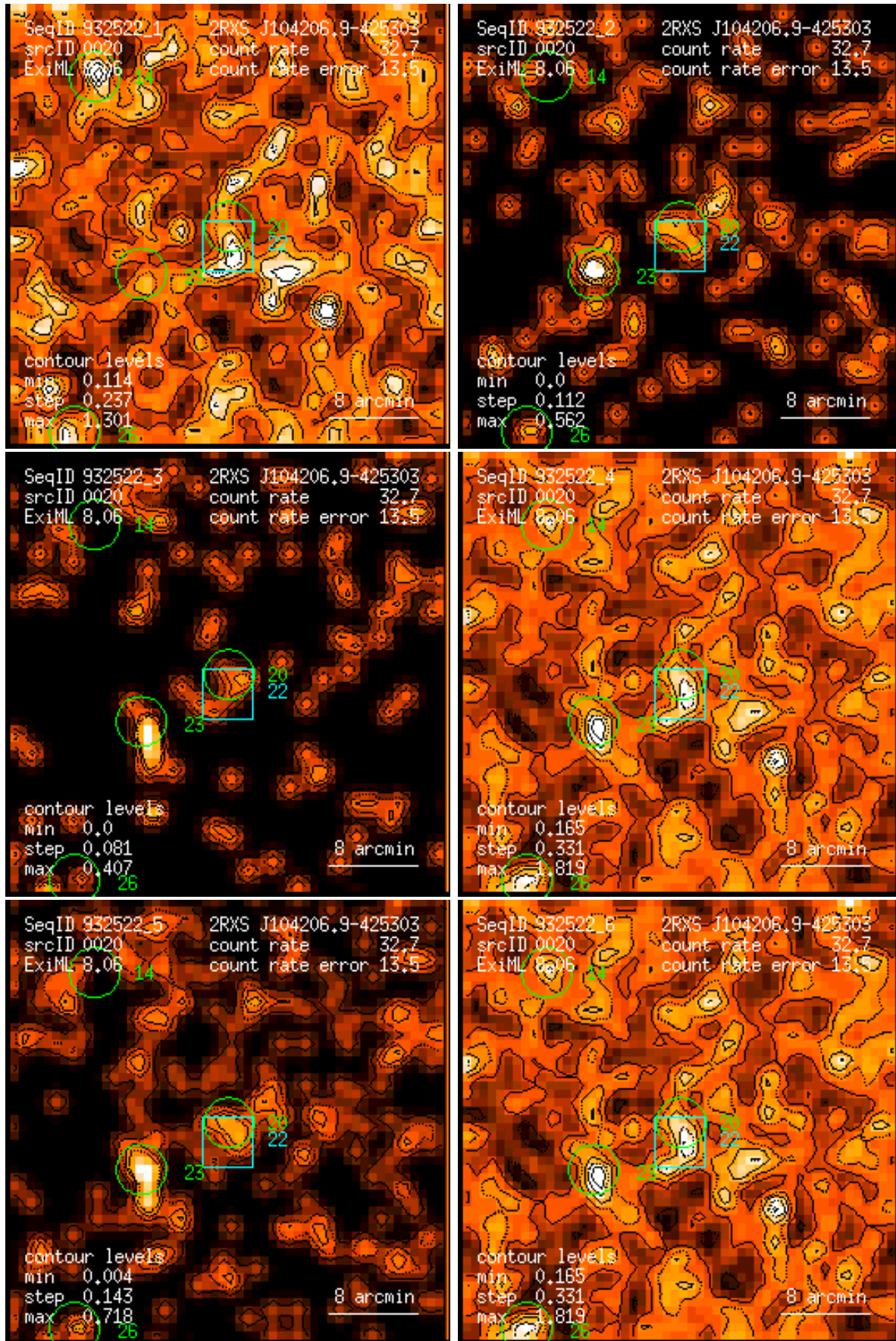
Figure 20: RASS 932522: detection 0020: band rate images, Gaussian filter: (1) PSPC channels 11 – 41, (2) 52 – 90, (3) 91 – 201, (4) 11 – 235, (5) 52 – 201, (6) 11 – 201. Broad band rates in counts/ks. Band rate contour levels in counts/ks/arcmin 2 .
