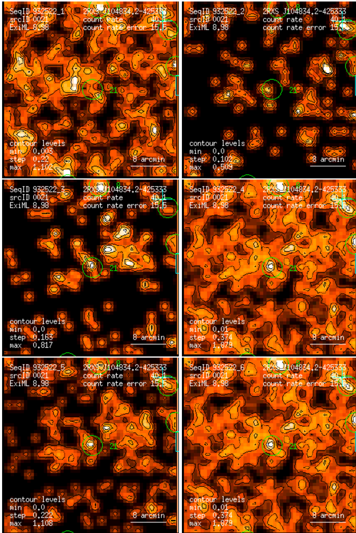
Figure 21: RASS 932522: detection 0021: band rate images, Gaussian filter: (1) PSPC channels 11 – 41, (2) 52 – 90, (3) 91 – 201, (4) 11 – 235, (5) 52 – 201, (6) 11 – 201. Broad band rates in counts/ks. Band rate contour levels in counts/ks/arcmin 2 .
