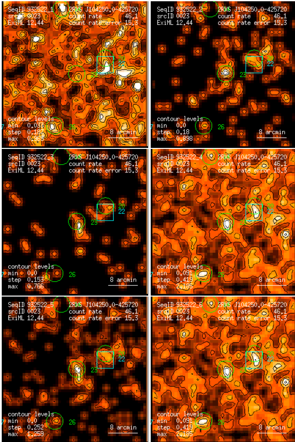
Figure 23: RASS 932522: detection 0023: band rate images, Gaussian filter: (1) PSPC channels 11 – 41, (2) 52 – 90, (3) 91 – 201, (4) 11 – 235, (5) 52 – 201, (6) 11 – 201. Broad band rates in counts/ks. Band rate contour levels in counts/ks/arcmin 2 .
