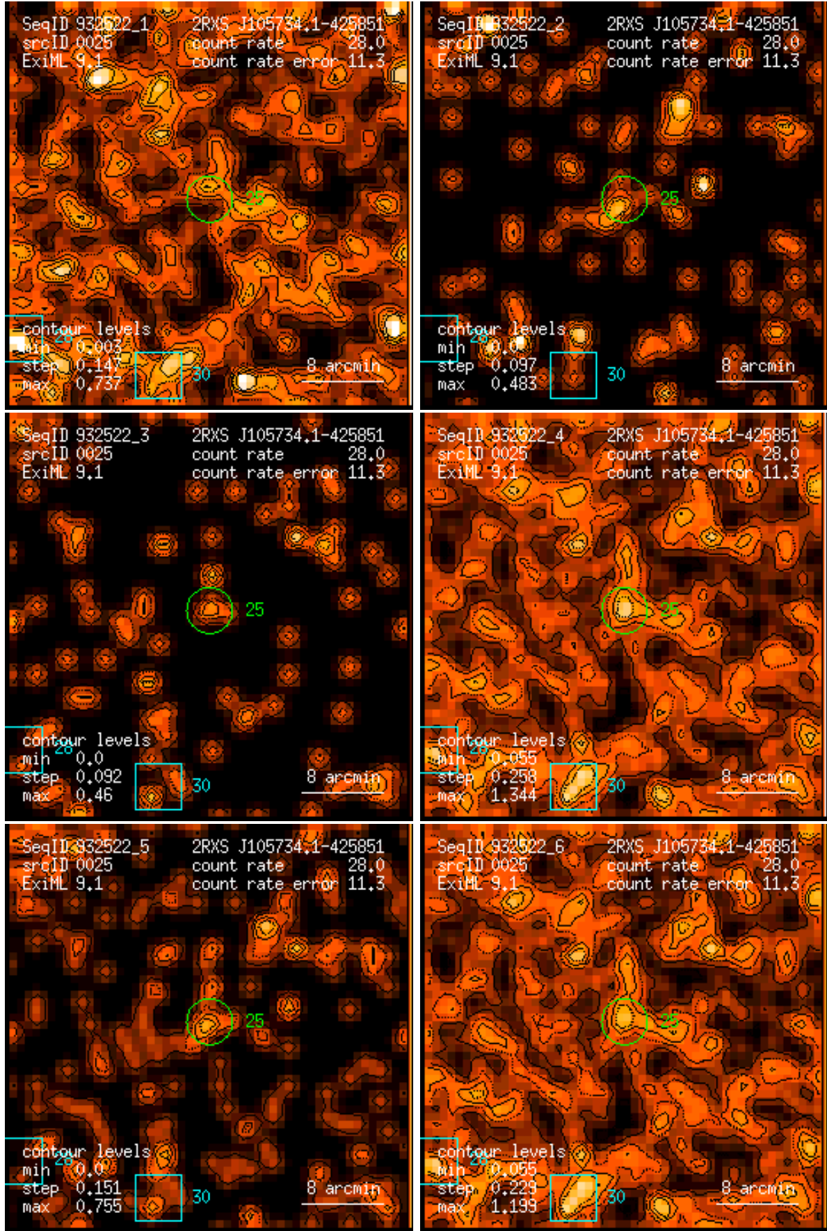
Figure 25: RASS 932522: detection 0025: band rate images, Gaussian filter: (1) PSPC channels 11 – 41, (2) 52 – 90, (3) 91 – 201, (4) 11 – 235, (5) 52 – 201, (6) 11 – 201. Broad band rates in counts/ks. Band rate contour levels in counts/ks/arcmin 2 .
