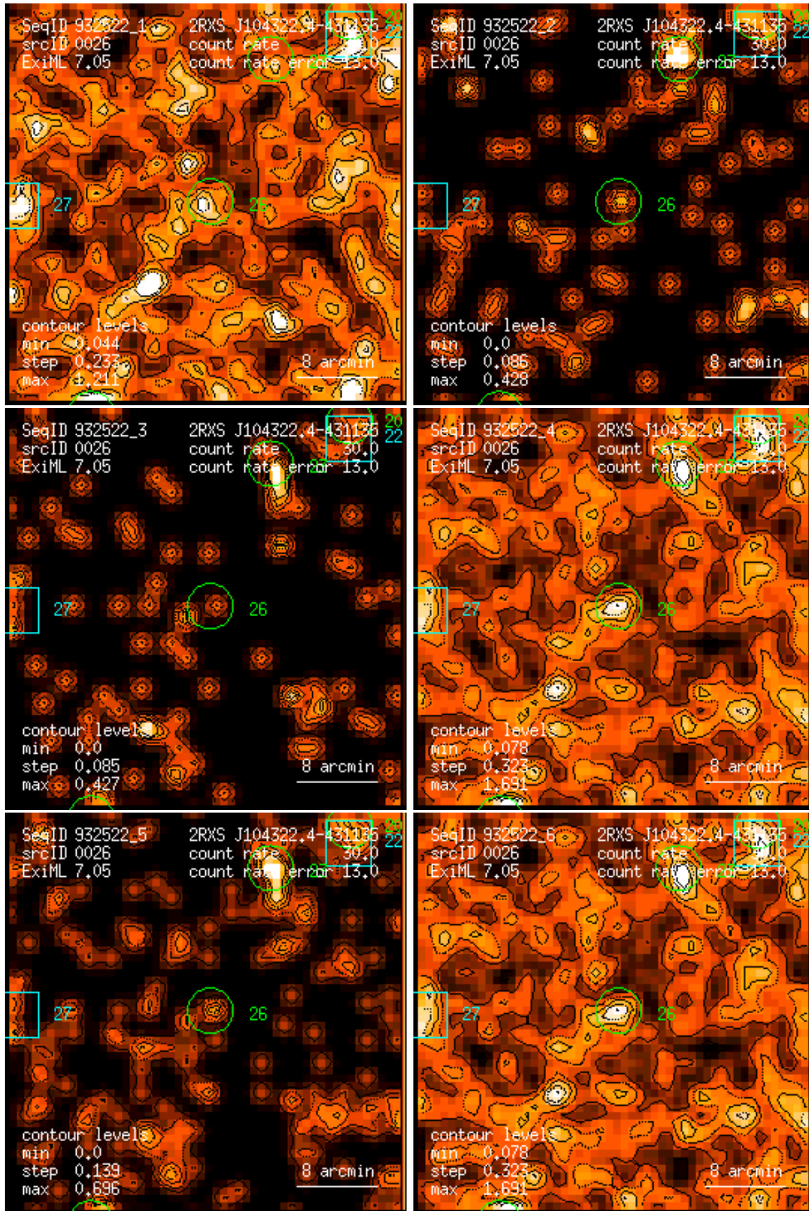
Figure 26: RASS 932522: detection 0026: band rate images, Gaussian filter: (1) PSPC channels 11 – 41, (2) 52 – 90, (3) 91 – 201, (4) 11 – 235, (5) 52 – 201, (6) 11 – 201. Broad band rates in counts/ks. Band rate contour levels in counts/ks/arcmin 2 .
