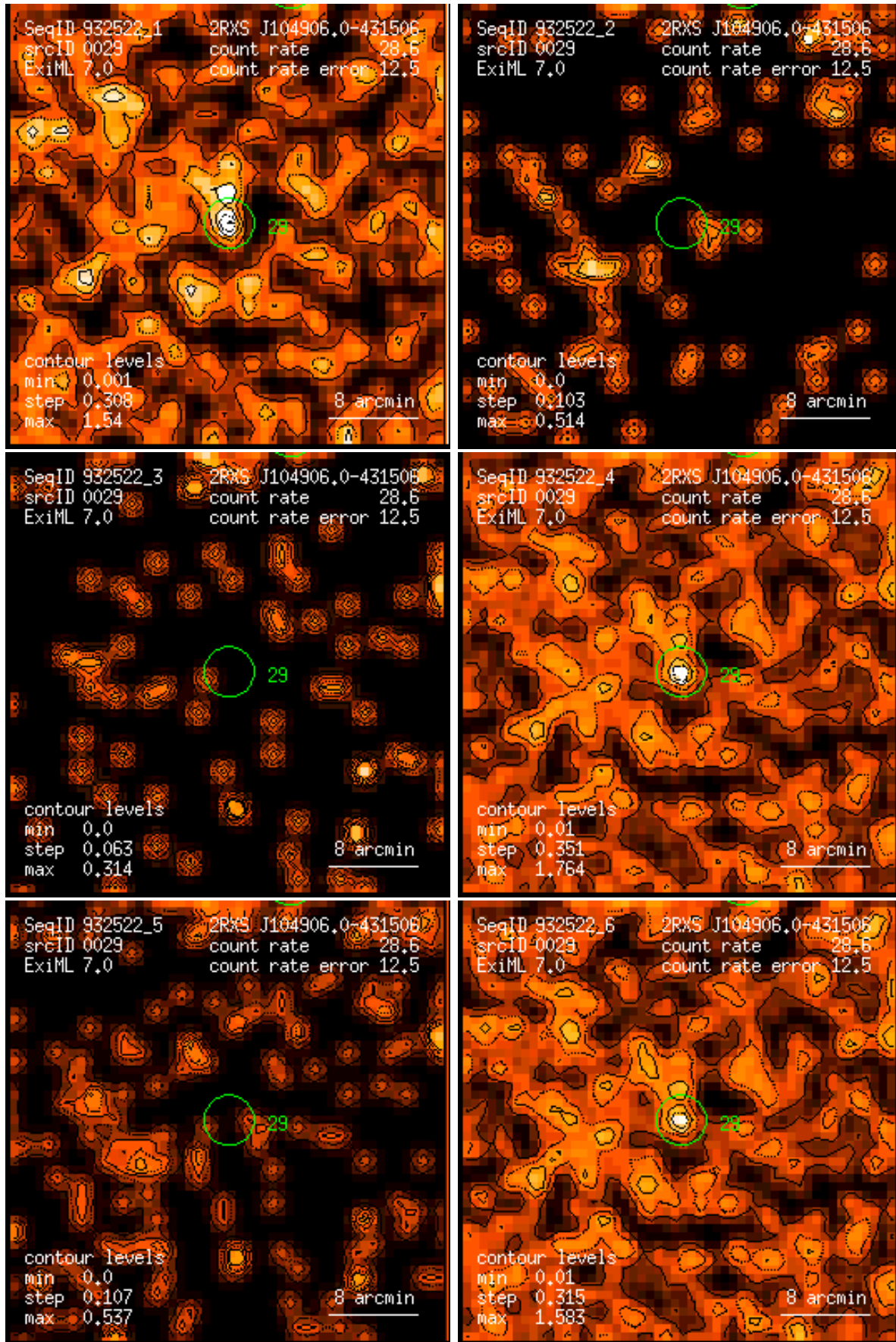
Figure 29: RASS 932522: detection 0029: band rate images, Gaussian filter: (1) PSPC channels 11 – 41, (2) 52 – 90, (3) 91 – 201, (4) 11 – 235, (5) 52 – 201, (6) 11 – 201. Broad band rates in counts/ks. Band rate contour levels in counts/ks/arcmin 2 .
