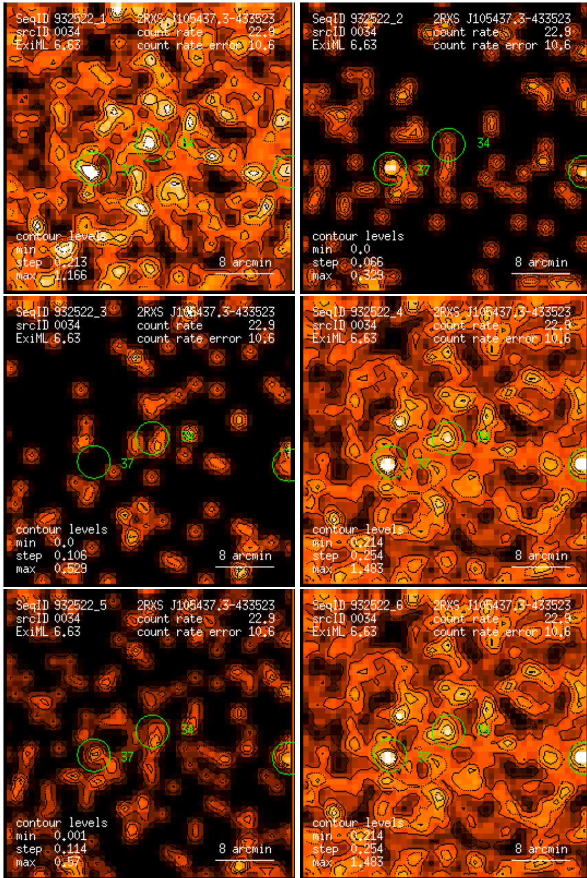
Figure 34: RASS 932522: detection 0034: band rate images, Gaussian filter: (1) PSPC channels 11 – 41, (2) 52 – 90, (3) 91 – 201, (4) 11 – 235, (5) 52 – 201, (6) 11 – 201. Broad band rates in counts/ks. Band rate contour levels in counts/ks/arcmin 2 .
