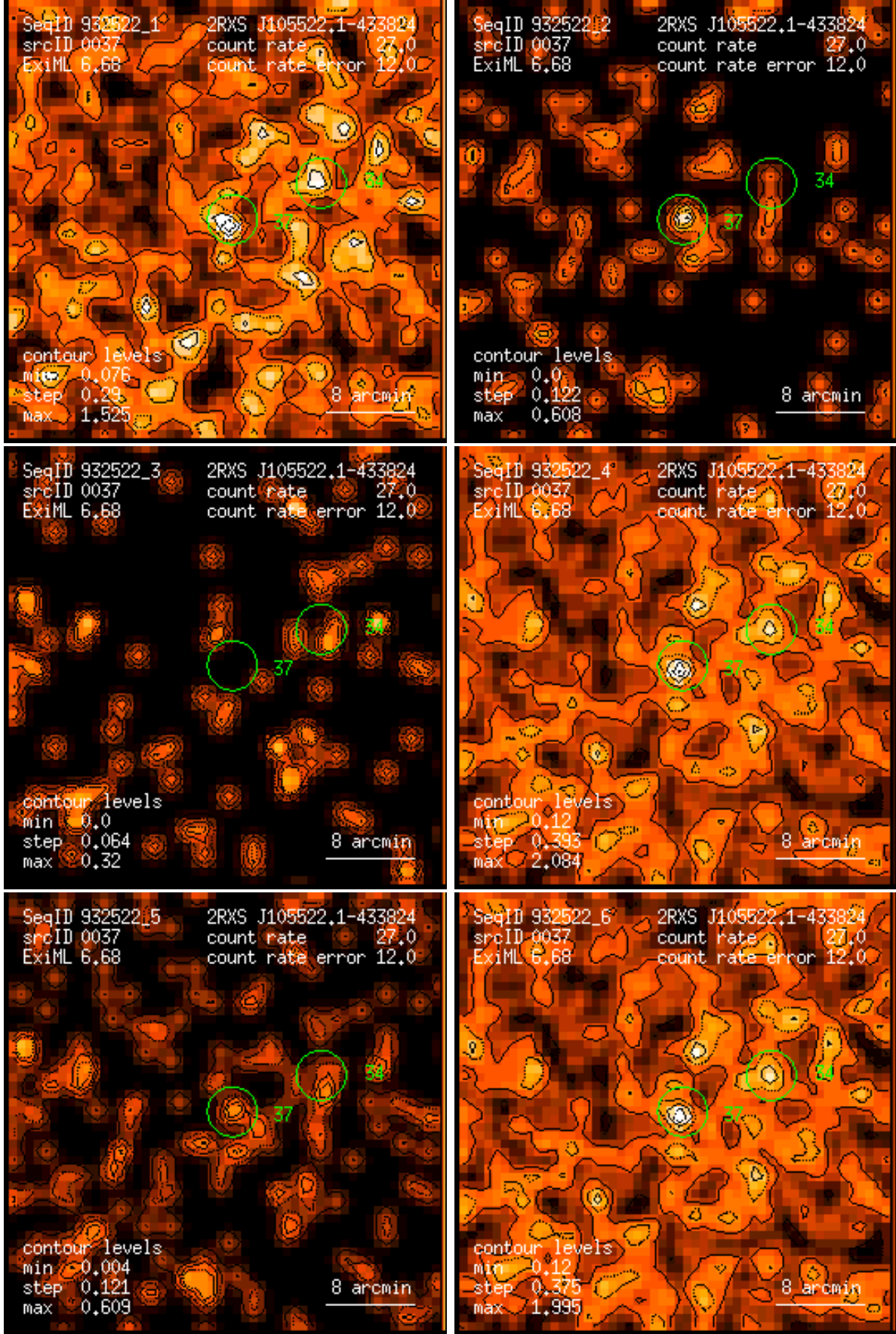
Figure 37: RASS 932522: detection 0037: band rate images, Gaussian filter: (1) PSPC channels 11 – 41, (2) 52 – 90, (3) 91 – 201, (4) 11 – 235, (5) 52 – 201, (6) 11 – 201. Broad band rates in counts/ks. Band rate contour levels in counts/ks/arcmin 2 .
