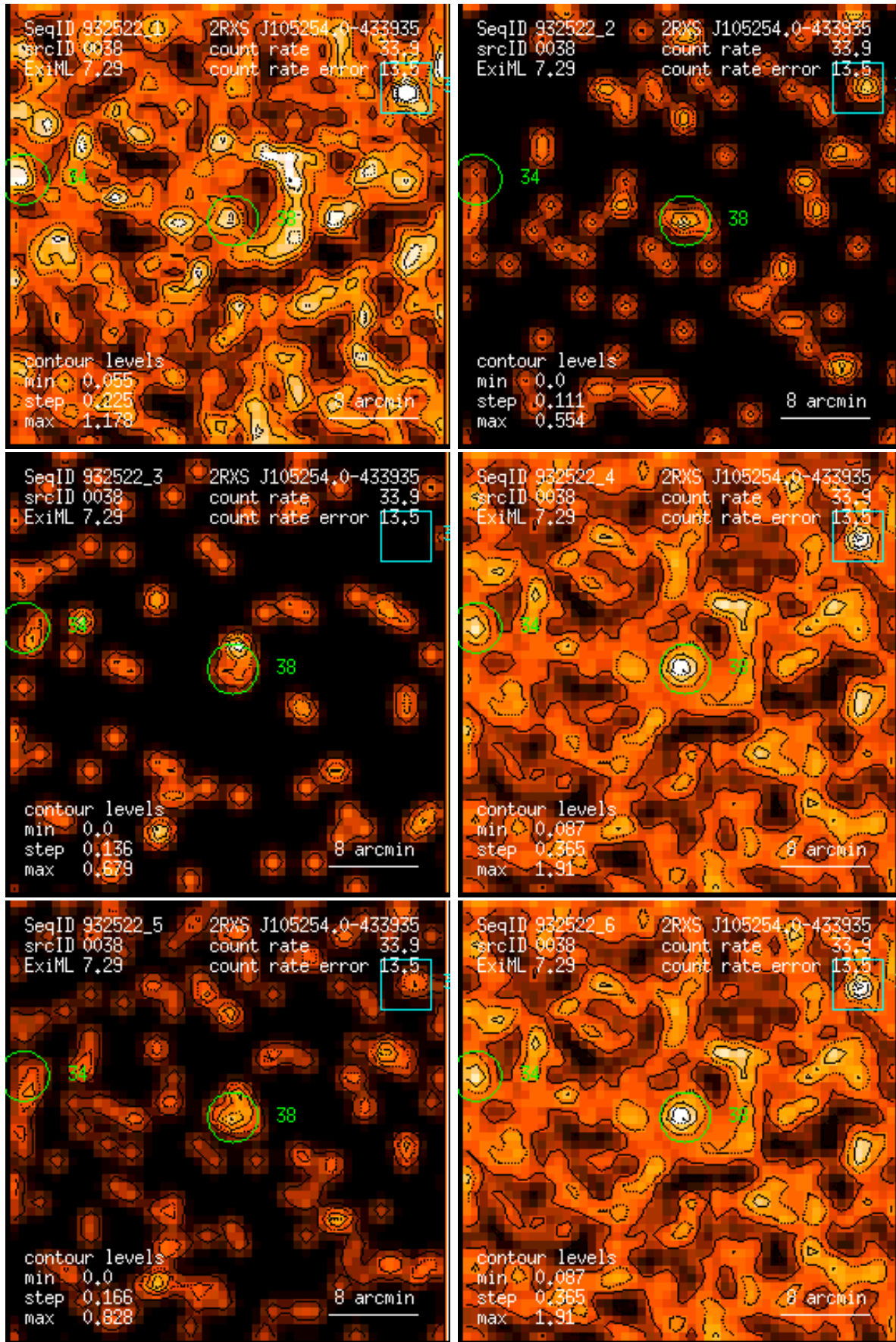
Figure 38: RASS 932522: detection 0038: band rate images, Gaussian filter: (1) PSPC channels 11 – 41, (2) 52 – 90, (3) 91 – 201, (4) 11 – 235, (5) 52 – 201, (6) 11 – 201. Broad band rates in counts/ks. Band rate contour levels in counts/ks/arcmin 2 .
