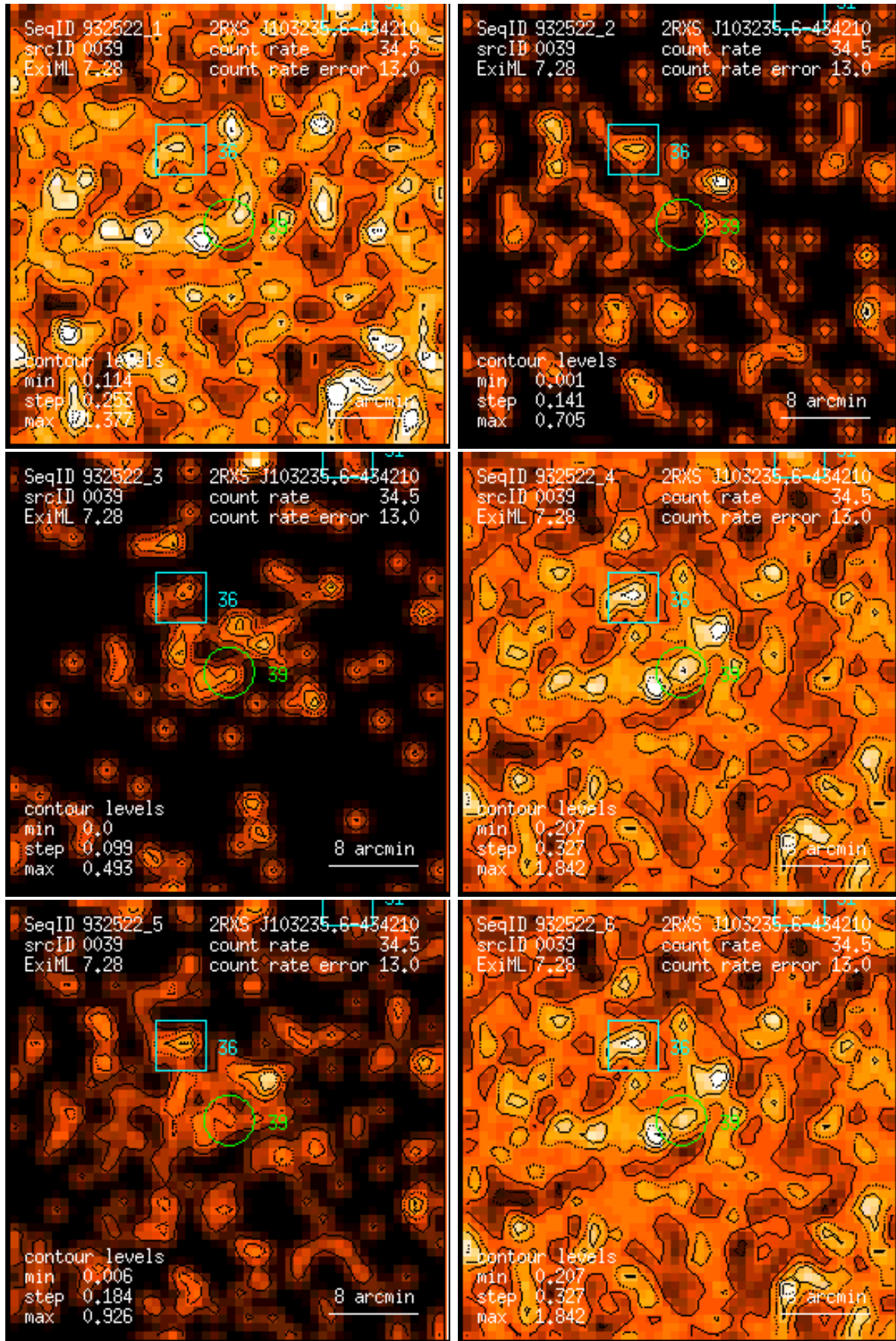
Figure 39: RASS 932522: detection 0039: band rate images, Gaussian filter: (1) PSPC channels 11 – 41, (2) 52 – 90, (3) 91 – 201, (4) 11 – 235, (5) 52 – 201, (6) 11 – 201. Broad band rates in counts/ks. Band rate contour levels in counts/ks/arcmin 2 .
