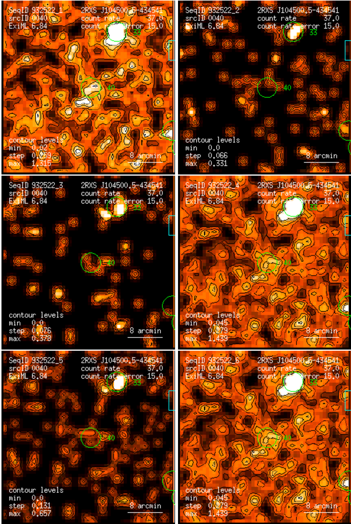
Figure 40: RASS 932522: detection 0040: band rate images, Gaussian filter: (1) PSPC channels 11 – 41, (2) 52 – 90, (3) 91 – 201, (4) 11 – 235, (5) 52 – 201, (6) 11 – 201. Broad band rates in counts/ks. Band rate contour levels in counts/ks/arcmin 2 .
