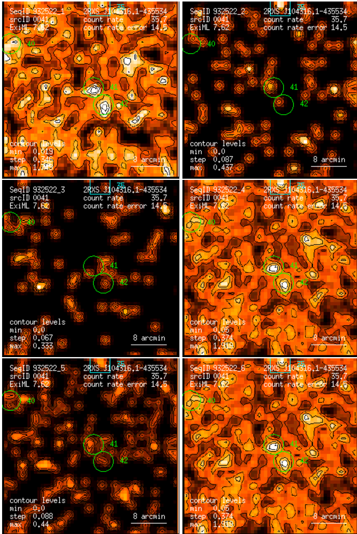
Figure 41: RASS 932522: detection 0041: band rate images, Gaussian filter: (1) PSPC channels 11 – 41, (2) 52 – 90, (3) 91 – 201, (4) 11 – 235, (5) 52 – 201, (6) 11 – 201. Broad band rates in counts/ks. Band rate contour levels in counts/ks/arcmin 2 .
