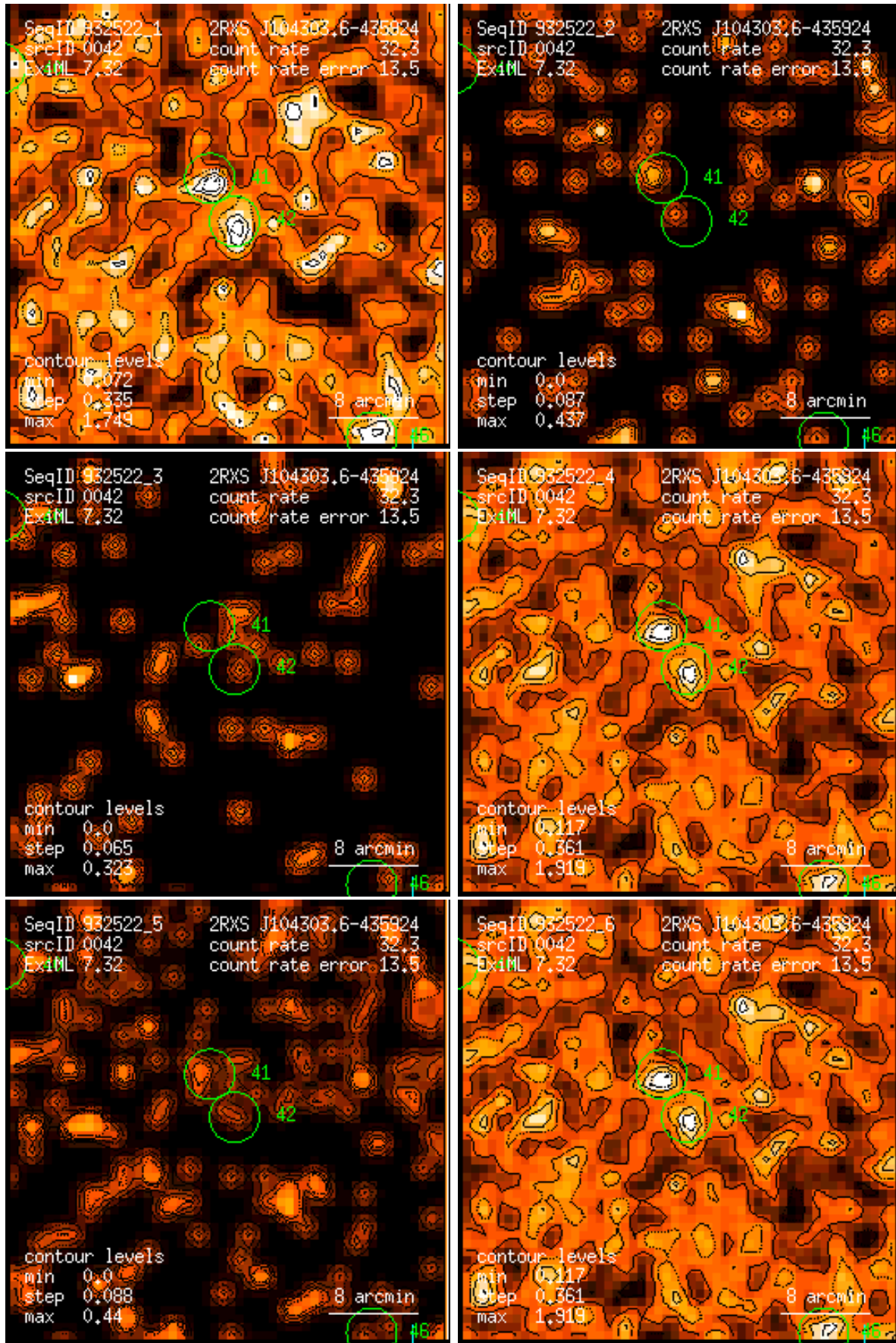
Figure 42: RASS 932522: detection 0042: band rate images, Gaussian filter: (1) PSPC channels 11 – 41, (2) 52 – 90, (3) 91 – 201, (4) 11 – 235, (5) 52 – 201, (6) 11 – 201. Broad band rates in counts/ks. Band rate contour levels in counts/ks/arcmin 2 .
