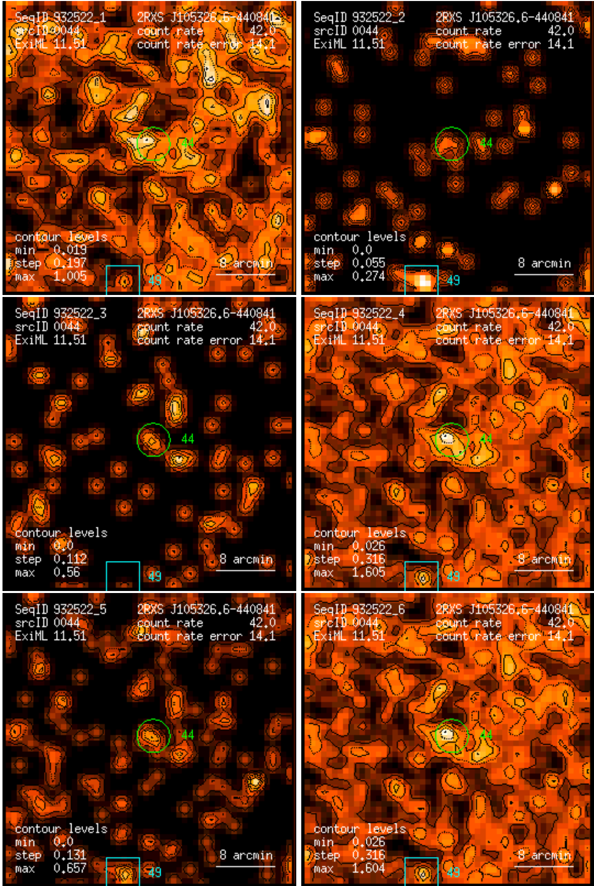
Figure 44: RASS 932522: detection 0044: band rate images, Gaussian filter: (1) PSPC channels 11 – 41, (2) 52 – 90, (3) 91 – 201, (4) 11 – 235, (5) 52 – 201, (6) 11 – 201. Broad band rates in counts/ks. Band rate contour levels in counts/ks/arcmin 2 .
