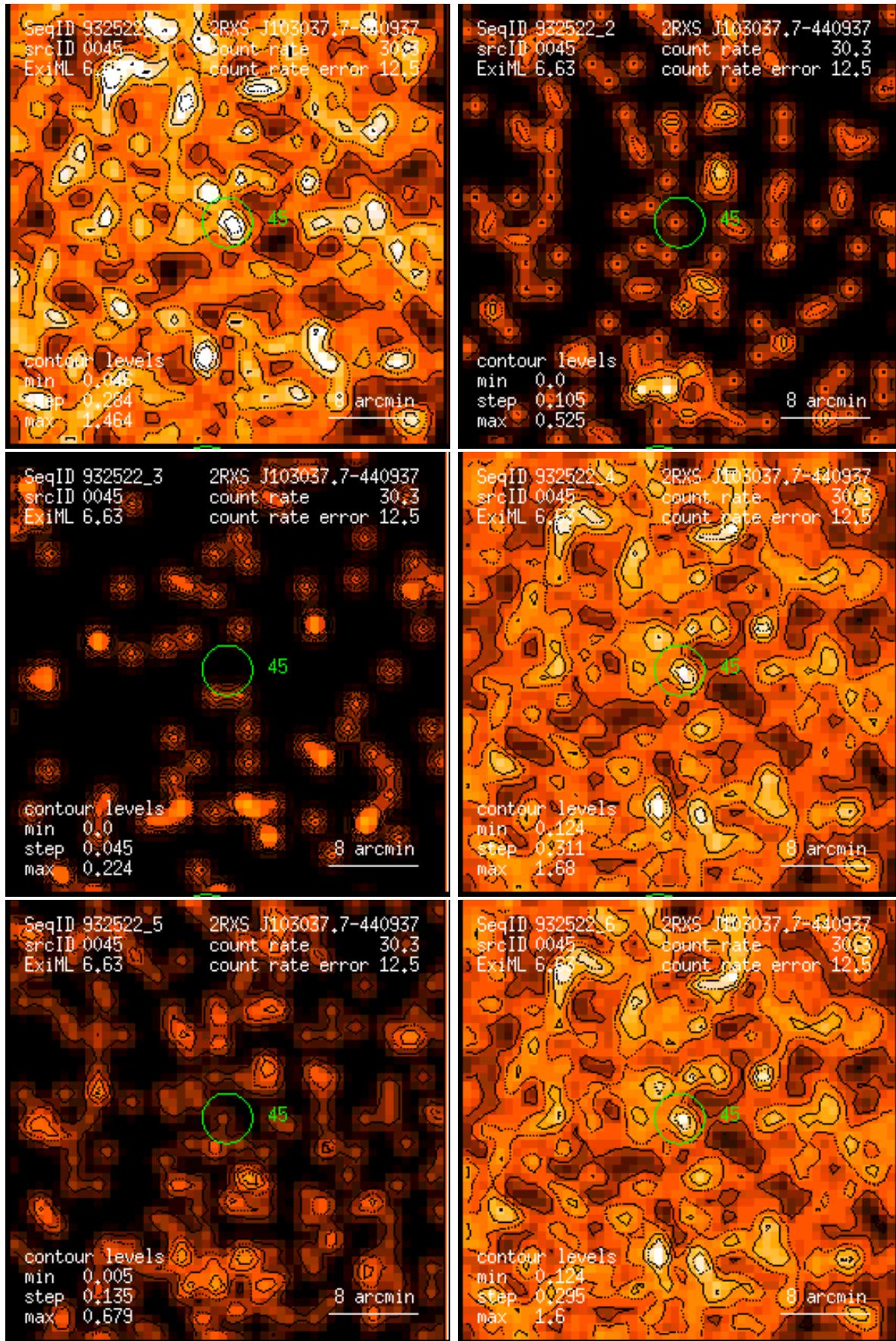
Figure 45: RASS 932522: detection 0045: band rate images, Gaussian filter: (1) PSPC channels 11 – 41, (2) 52 – 90, (3) 91 – 201, (4) 11 – 235, (5) 52 – 201, (6) 11 – 201. Broad band rates in counts/ks. Band rate contour levels in counts/ks/arcmin 2 .
