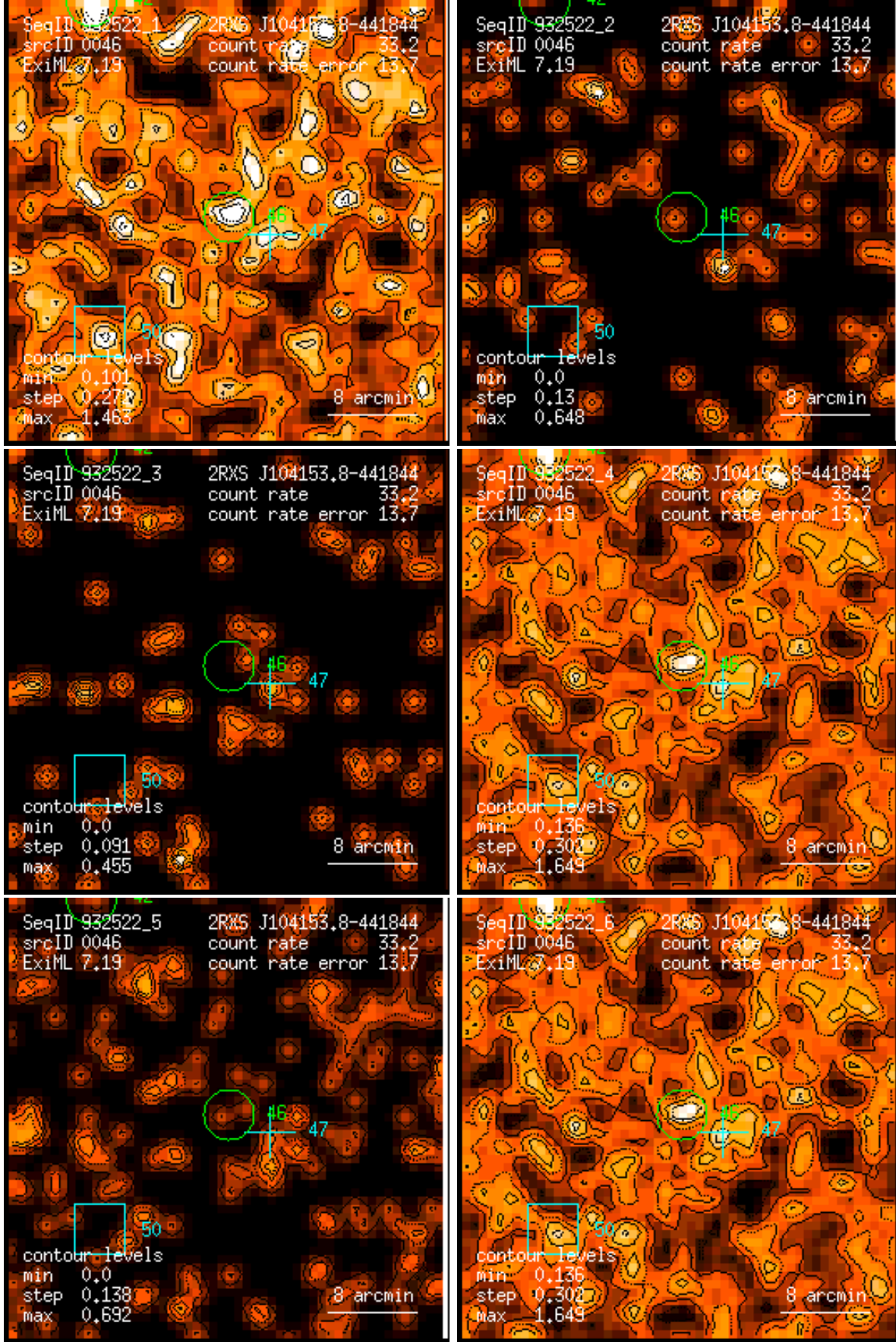
Figure 46: RASS 932522: detection 0046: band rate images, Gaussian filter: (1) PSPC channels 11 – 41, (2) 52 – 90, (3) 91 – 201, (4) 11 – 235, (5) 52 – 201, (6) 11 – 201. Broad band rates in counts/ks. Band rate contour levels in counts/ks/arcmin 2 .
