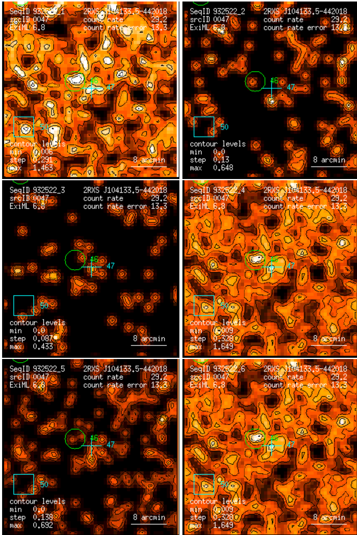
Figure 47: RASS 932522: detection 0047: band rate images, Gaussian filter: (1) PSPC channels 11 – 41, (2) 52 – 90, (3) 91 – 201, (4) 11 – 235, (5) 52 – 201, (6) 11 – 201. Broad band rates in counts/ks. Band rate contour levels in counts/ks/arcmin 2 .
