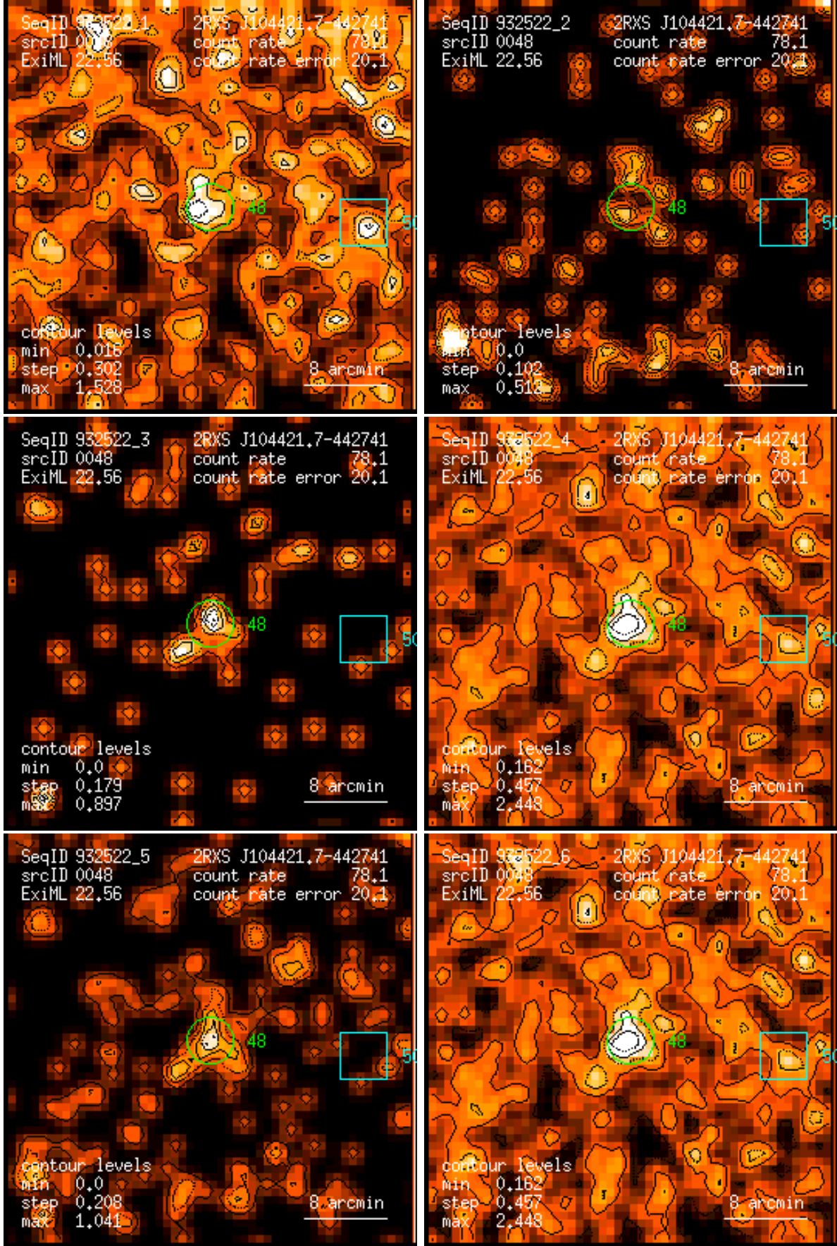
Figure 48: RASS 932522: detection 0048: band rate images, Gaussian filter: (1) PSPC channels 11 – 41, (2) 52 – 90, (3) 91 – 201, (4) 11 – 235, (5) 52 – 201, (6) 11 – 201. Broad band rates in counts/ks. Band rate contour levels in counts/ks/arcmin 2 .
