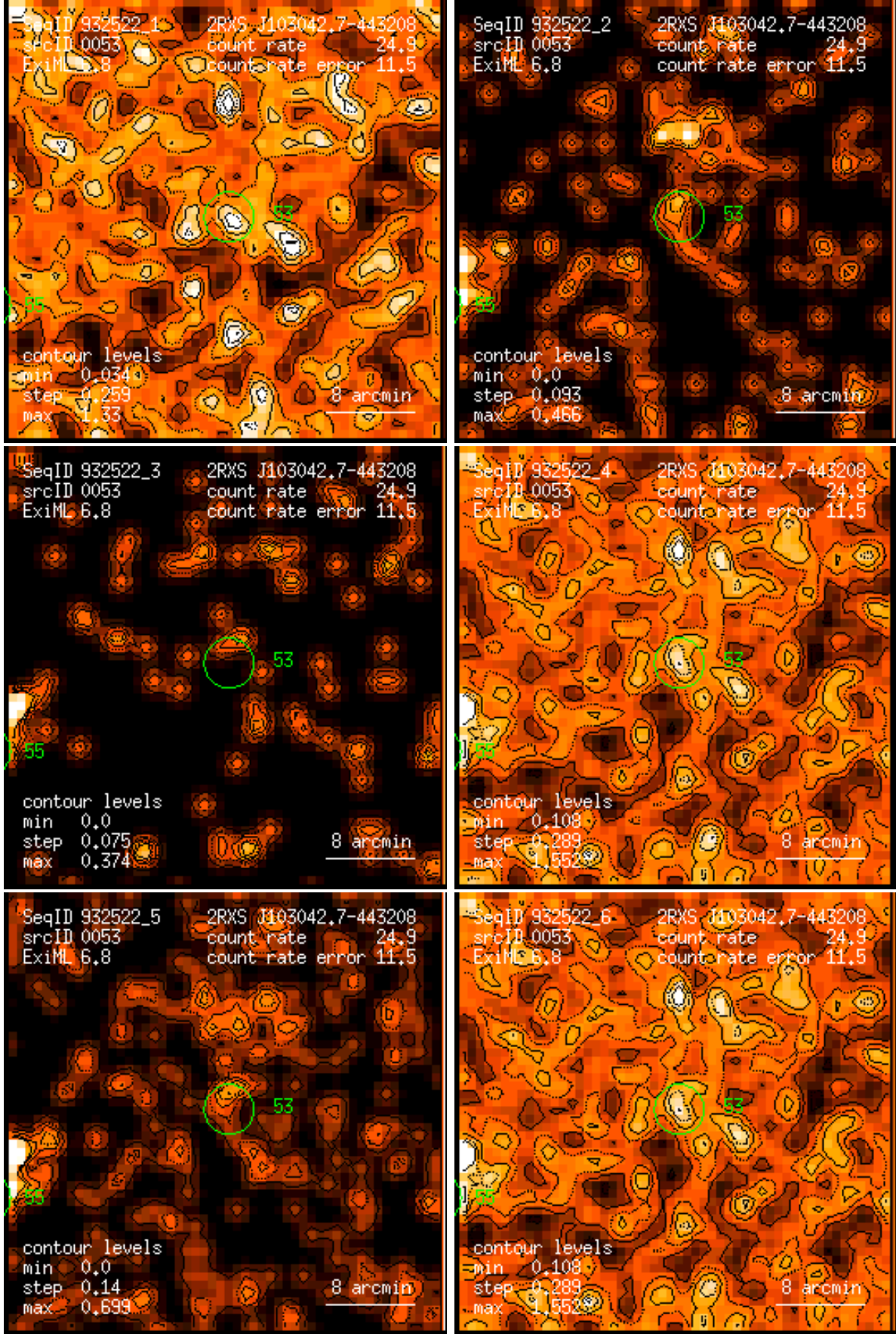
Figure 53: RASS 932522: detection 0053: band rate images, Gaussian filter: (1) PSPC channels 11 – 41, (2) 52 – 90, (3) 91 – 201, (4) 11 – 235, (5) 52 – 201, (6) 11 – 201. Broad band rates in counts/ks. Band rate contour levels in counts/ks/arcmin 2 .
