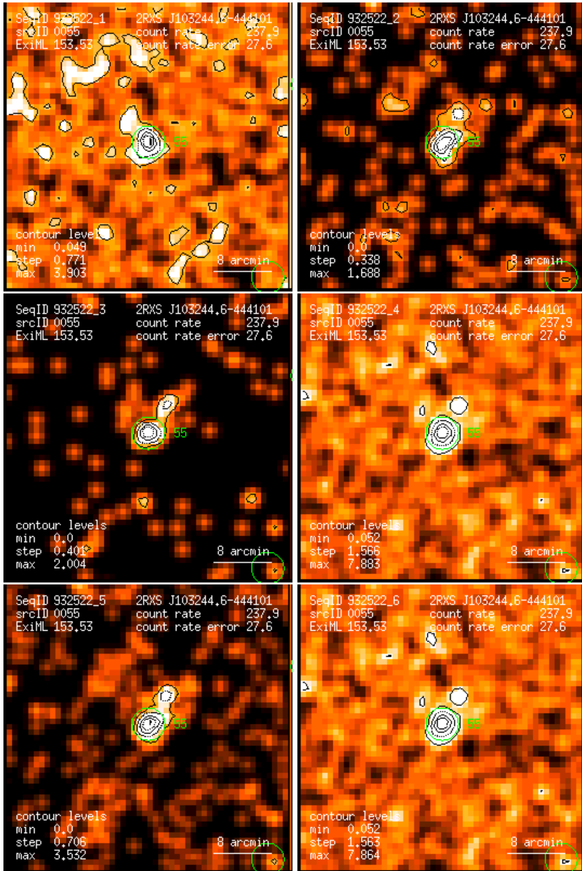
Figure 55: RASS 932522: detection 0055: band rate images, Gaussian filter: (1) PSPC channels 11 – 41, (2) 52 – 90, (3) 91 – 201, (4) 11 – 235, (5) 52 – 201, (6) 11 – 201. Broad band rates in counts/ks. Band rate contour levels in counts/ks/arcmin 2 .
