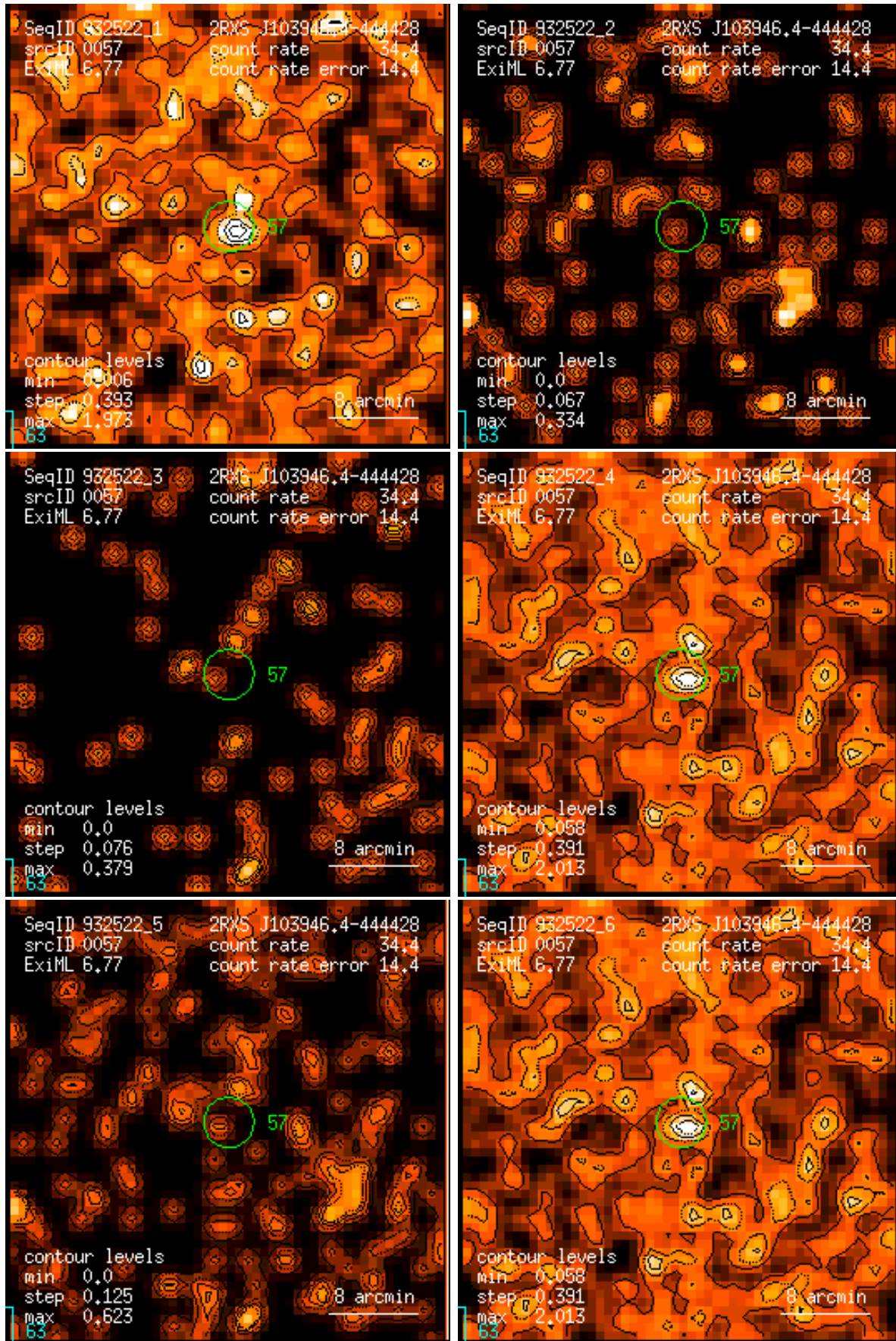
Figure 57: RASS 932522: detection 0057: band rate images, Gaussian filter: (1) PSPPC channels 11 – 41, (2) 52 – 90, (3) 91 – 201, (4) 11 – 235, (5) 52 – 201, (6) 11 – 201. Broad band rates in counts/ks. Band rate contour levels in counts/ks/arcmin 2 .
