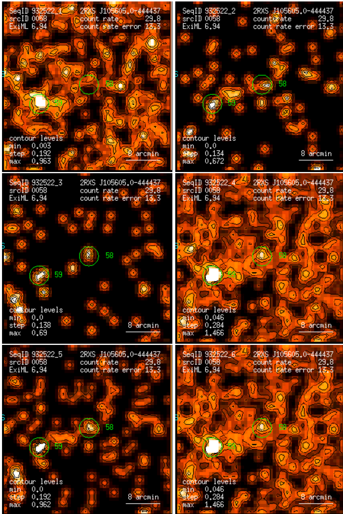
Figure 58: RASS 932522: detection 0058: band rate images, Gaussian filter: (1) PSPC channels 11 – 41, (2) 52 – 90, (3) 91 – 201, (4) 11 – 235, (5) 52 – 201, (6) 11 – 201. Broad band rates in counts/ks. Band rate contour levels in counts/ks/arcmin 2 .
