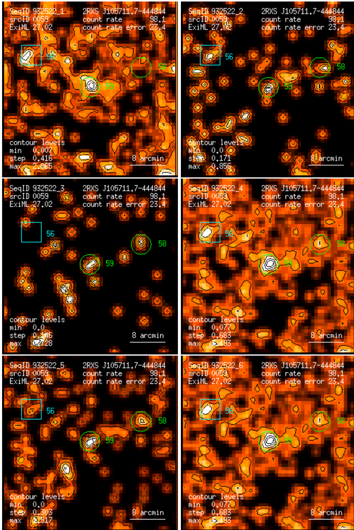
Figure 59: RASS 932522: detection 0059: band rate images, Gaussian filter: (1) PSPC channels 11 – 41, (2) 52 – 90, (3) 91 – 201, (4) 11 – 235, (5) 52 – 201, (6) 11 – 201. Broad band rates in counts/ks. Band rate contour levels in counts/ks/arcmin 2 .
