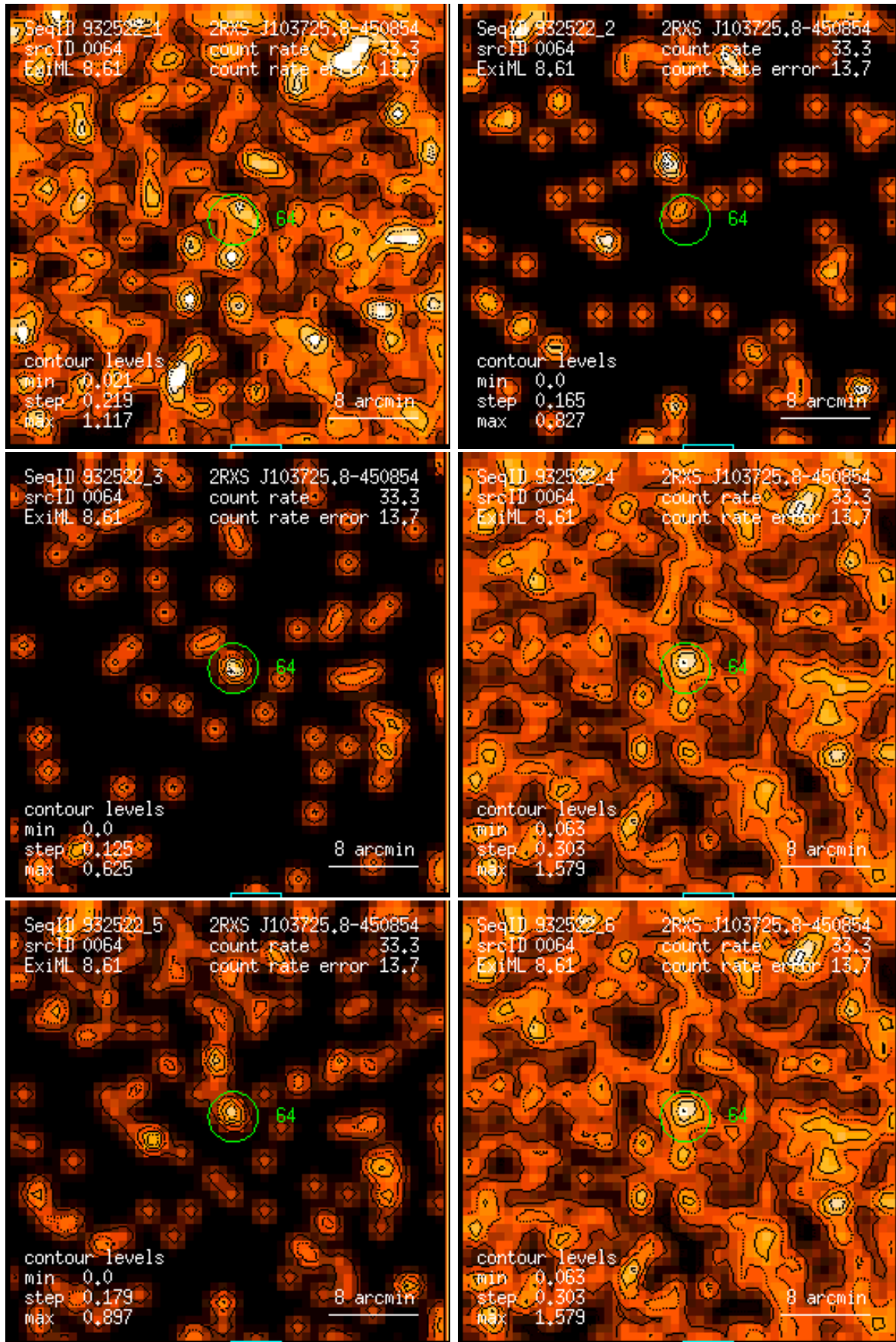
Figure 64: RASS 932522: detection 0064: band rate images, Gaussian filter: (1) PSPC channels 11 – 41, (2) 52 – 90, (3) 91 – 201, (4) 11 – 235, (5) 52 – 201, (6) 11 – 201. Broad band rates in counts/ks. Band rate contour levels in counts/ks/arcmin 2 .
