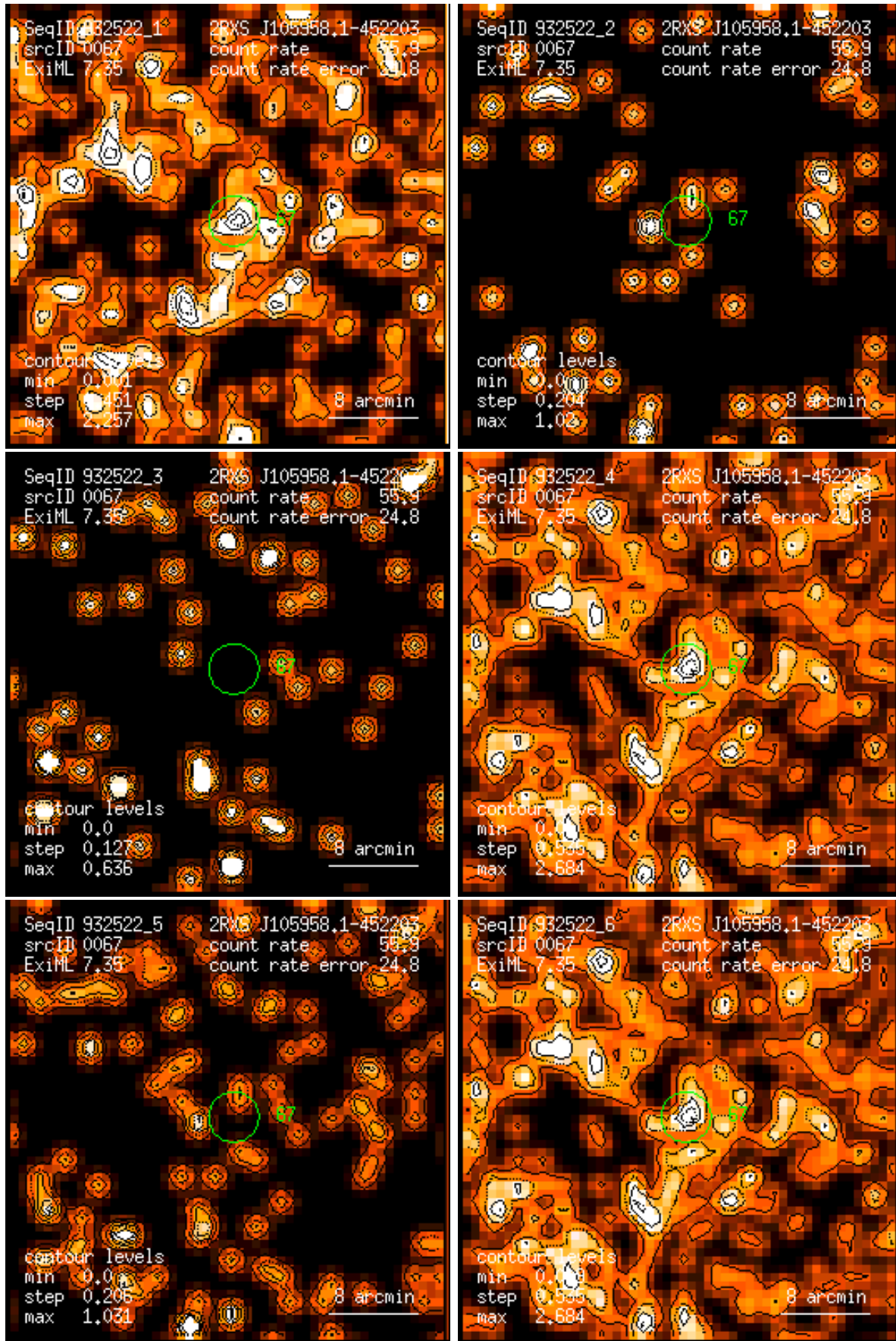
Figure 67: RASS 932522: detection 0067: band rate images, Gaussian filter: (1) PSPC channels 11 – 41, (2) 52 – 90, (3) 91 – 201, (4) 11 – 235, (5) 52 – 201, (6) 11 – 201. Broad band rates in counts/ks. Band rate contour levels in counts/ks/arcmin 2 .
