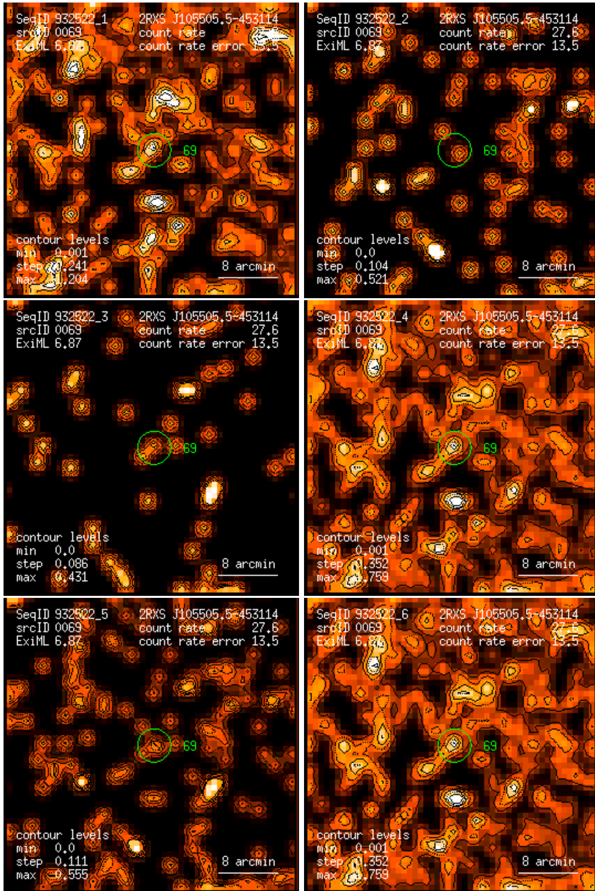
Figure 69: RASS 932522: detection 0069: band rate images, Gaussian filter: (1) PSPC channels 11 – 41, (2) 52 – 90, (3) 91 – 201, (4) 11 – 235, (5) 52 – 201, (6) 11 – 201. Broad band rates in counts/ks. Band rate contour levels in counts/ks/arcmin 2 .
