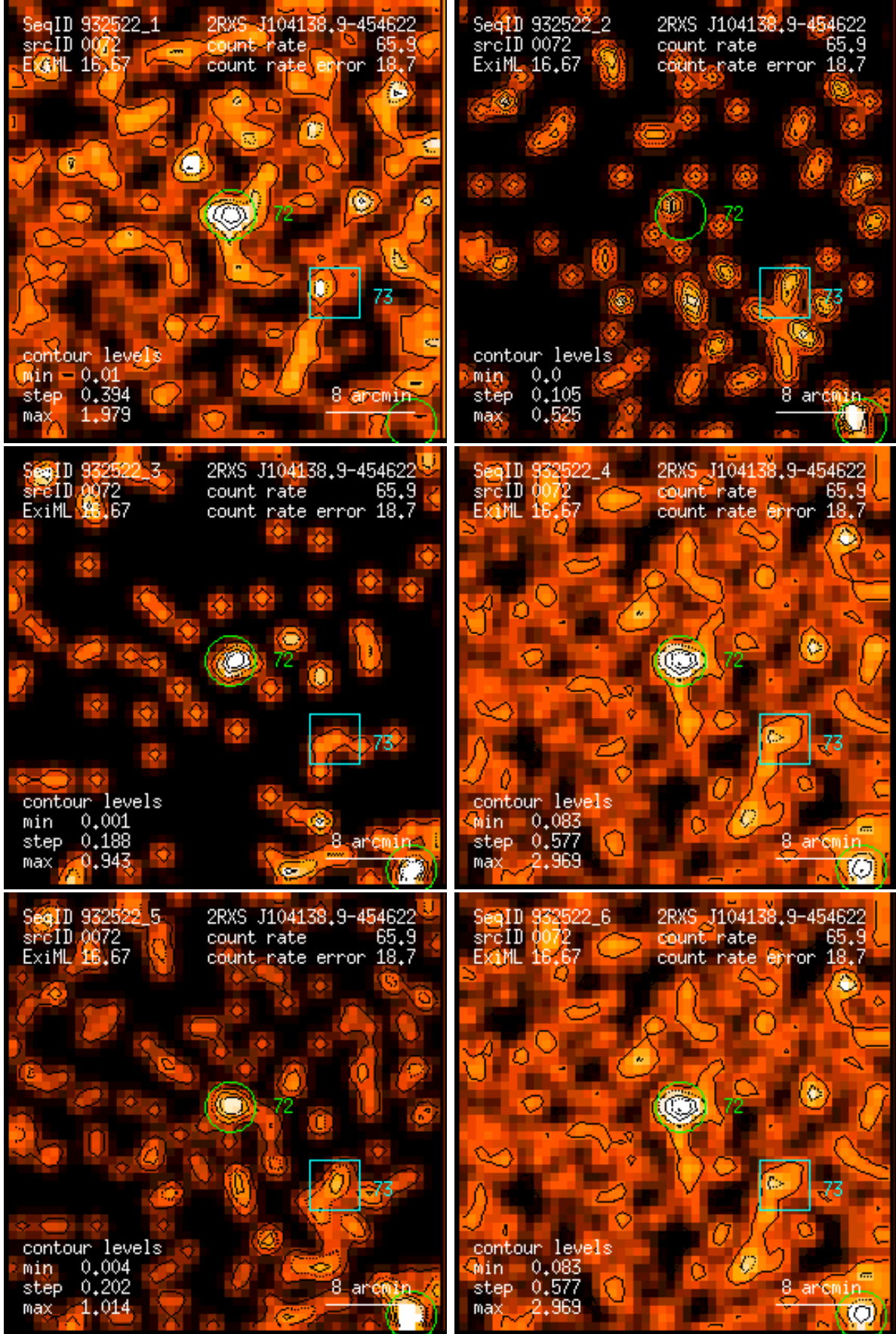
Figure 72: RASS 932522: detection 0072: band rate images, Gaussian filter: (1) PSPC channels 11 – 41, (2) 52 – 90, (3) 91 – 201, (4) 11 – 235, (5) 52 – 201, (6) 11 – 201. Broad band rates in counts/ks. Band rate contour levels in counts/ks/arcmin 2 .
