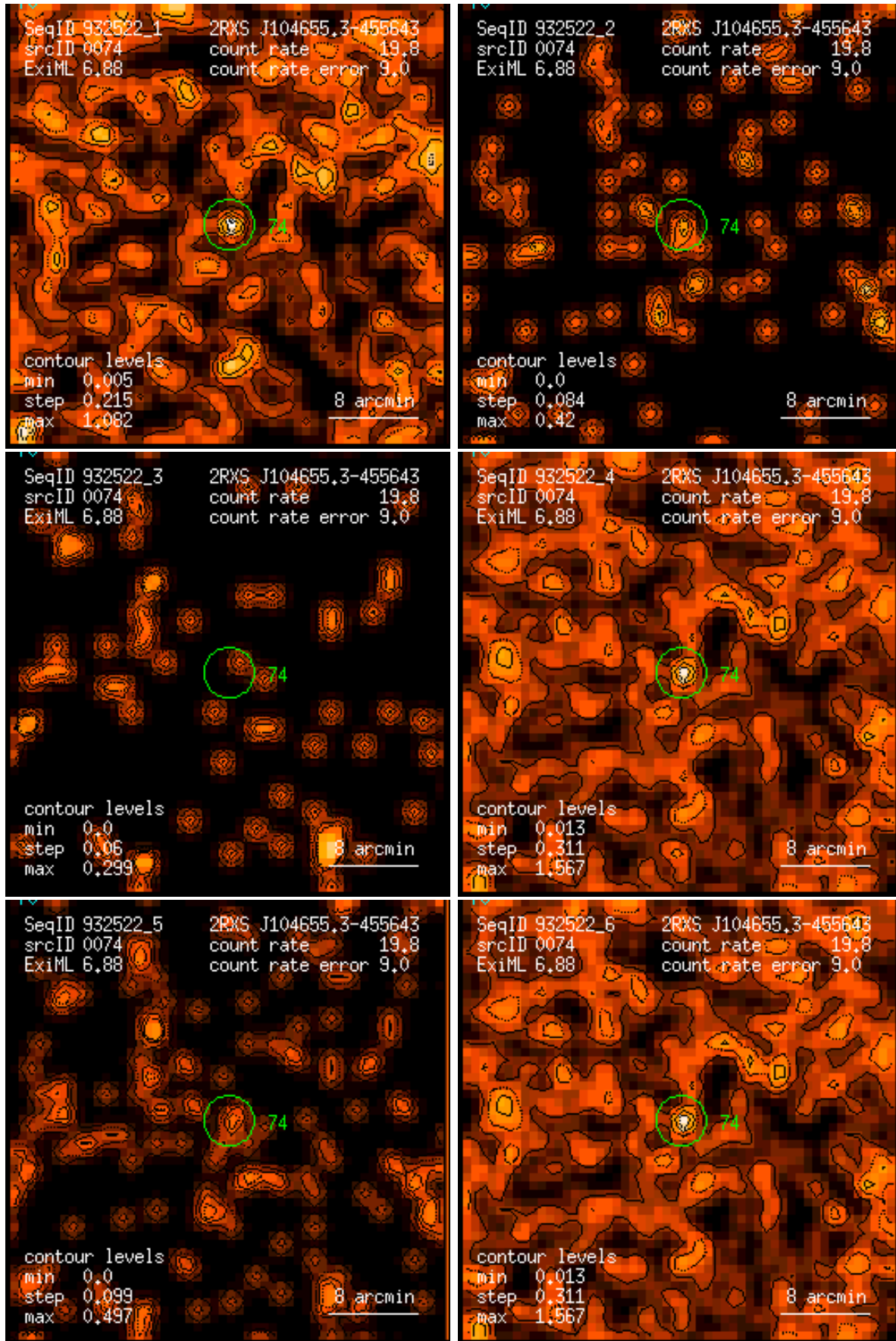
Figure 74: RASS 932522: detection 0074: band rate images, Gaussian filter: (1) PSPC channels 11 – 41, (2) 52 – 90, (3) 91 – 201, (4) 11 – 235, (5) 52 – 201, (6) 11 – 201. Broad band rates in counts/ks. Band rate contour levels in counts/ks/arcmin 2 .
