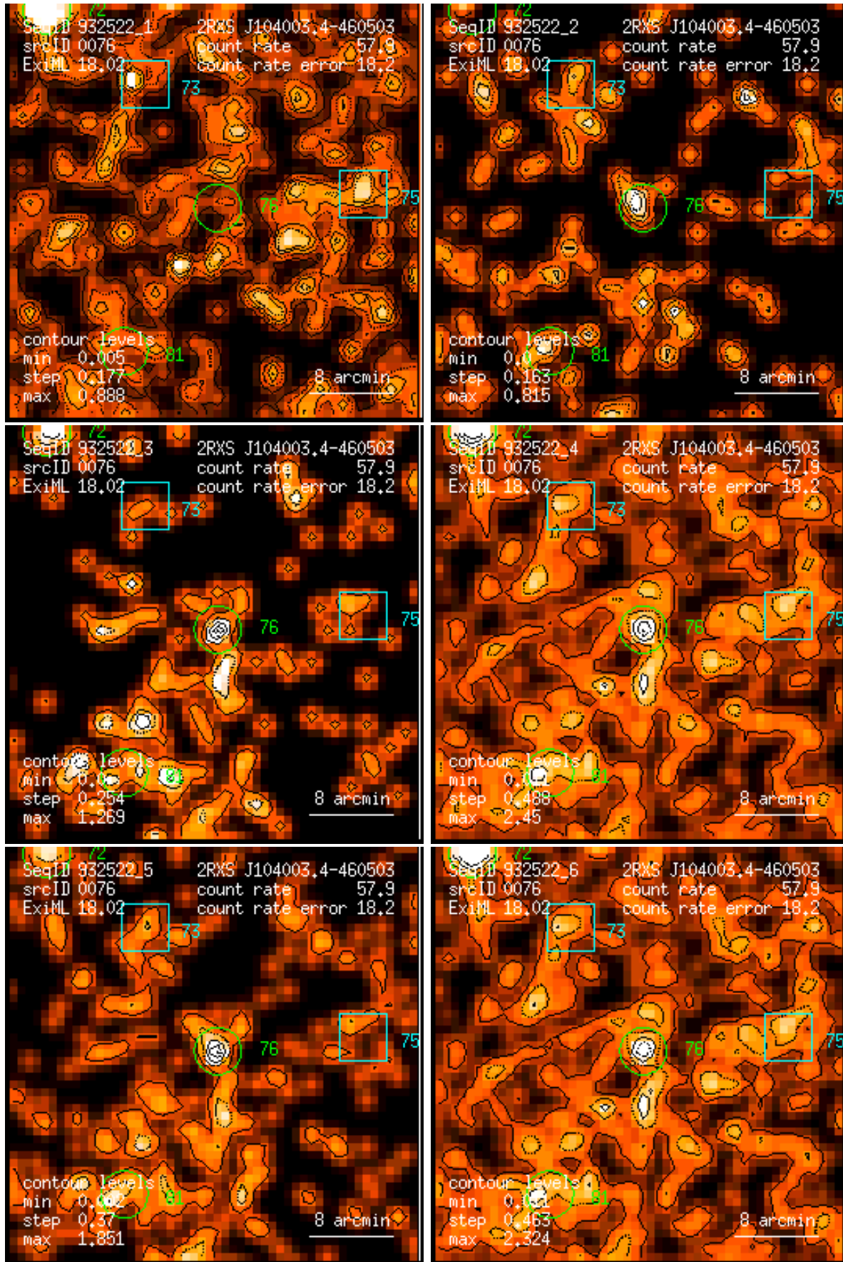
Figure 76: RASS 932522: detection 0076: band rate images, Gaussian filter: (1) PSPC channels 11 – 41, (2) 52 – 90, (3) 91 – 201, (4) 11 – 235, (5) 52 – 201, (6) 11 – 201. Broad band rates in counts/ks. Band rate contour levels in counts/ks/arcmin 2 .
