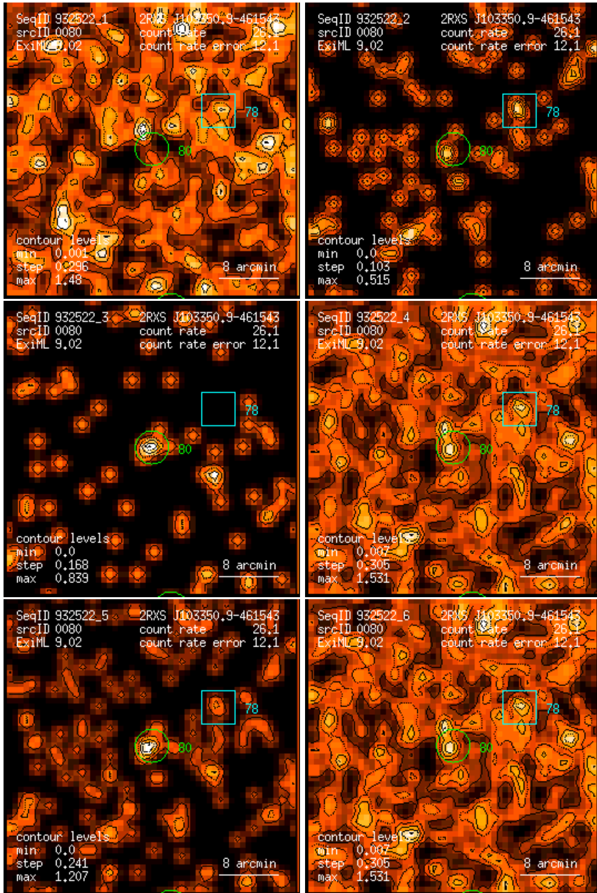
Figure 80: RASS 932522: detection 0080: band rate images, Gaussian filter: (1) PSPC channels 11 – 41, (2) 52 – 90, (3) 91 – 201, (4) 11 – 235, (5) 52 – 201, (6) 11 – 201. Broad band rates in counts/ks. Band rate contour levels in counts/ks/arcmin 2 .
