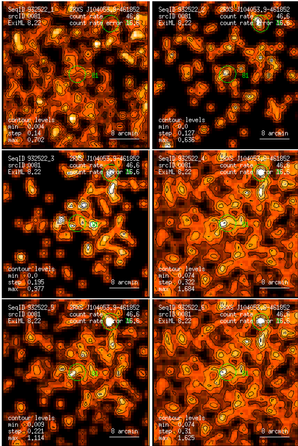
Figure 81: RASS 932522: detection 0081: band rate images, Gaussian filter: (1) PSPC channels 11 – 41, (2) 52 – 90, (3) 91 – 201, (4) 11 – 235, (5) 52 – 201, (6) 11 – 201. Broad band rates in counts/ks. Band rate contour levels in counts/ks/arcmin 2 .
