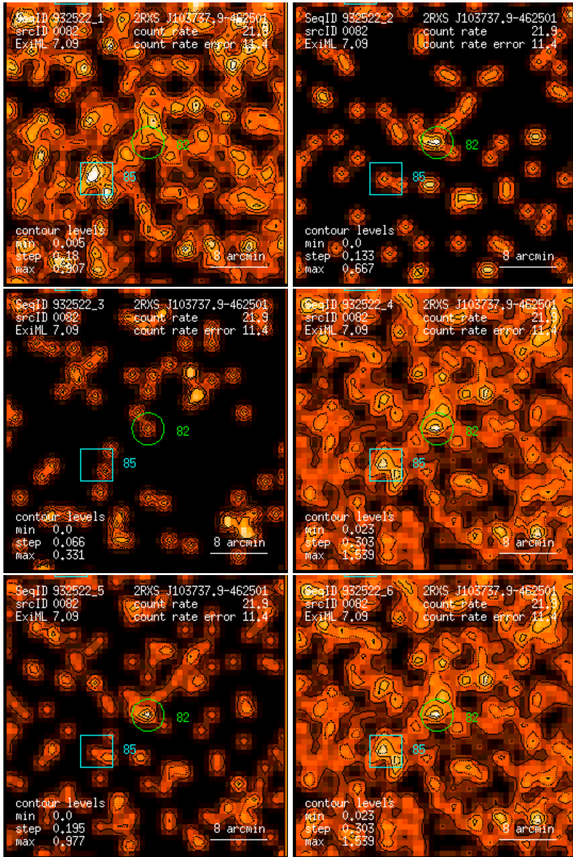
Figure 82: RASS 932522: detection 0082: band rate images, Gaussian filter: (1) PSPC channels 11 – 41, (2) 52 – 90, (3) 91 – 201, (4) 11 – 235, (5) 52 – 201, (6) 11 – 201. Broad band rates in counts/ks. Band rate contour levels in counts/ks/arcmin 2 .
