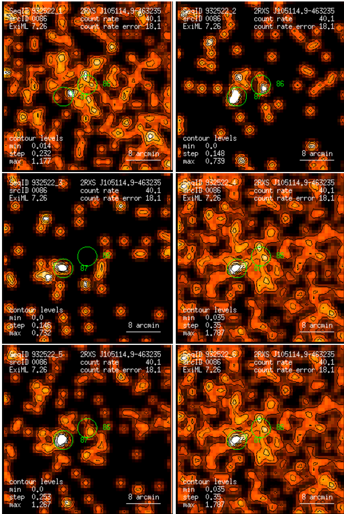
Figure 86: RASS 932522: detection 0086: band rate images, Gaussian filter: (1) PSPC channels 11 – 41, (2) 52 – 90, (3) 91 – 201, (4) 11 – 235, (5) 52 – 201, (6) 11 – 201. Broad band rates in counts/ks. Band rate contour levels in counts/ks/arcmin 2 .
