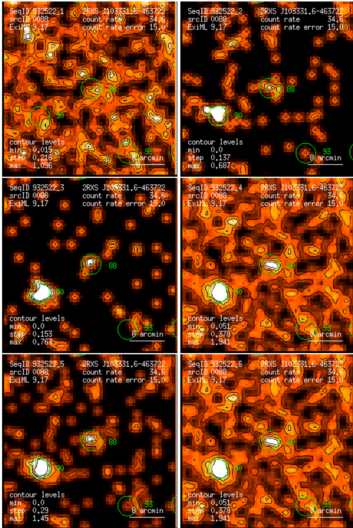
Figure 88: RASS 932522: detection 0088: band rate images, Gaussian filter: (1) PSPC channels 11 – 41, (2) 52 – 90, (3) 91 – 201, (4) 11 – 235, (5) 52 – 201, (6) 11 – 201. Broad band rates in counts/ks. Band rate contour levels in counts/ks/arcmin 2 .
