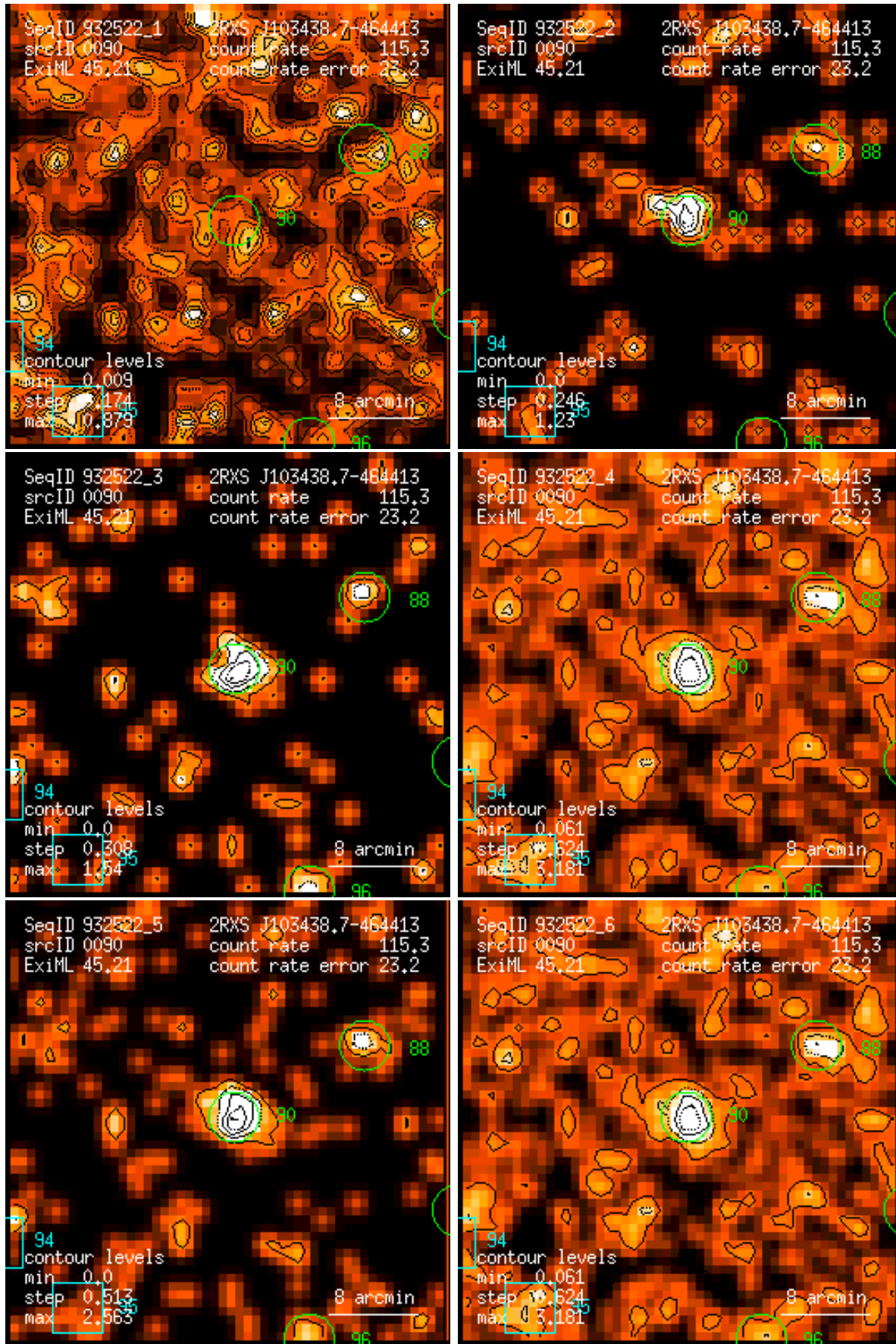
Figure 90: RASS 932522: detection 0090: band rate images, Gaussian filter: (1) PSPC channels 11 – 41, (2) 52 – 90, (3) 91 – 201, (4) 11 – 235, (5) 52 – 201, (6) 11 – 201. Broad band rates in counts/ks. Band rate contour levels in counts/ks/arcmin 2 .
