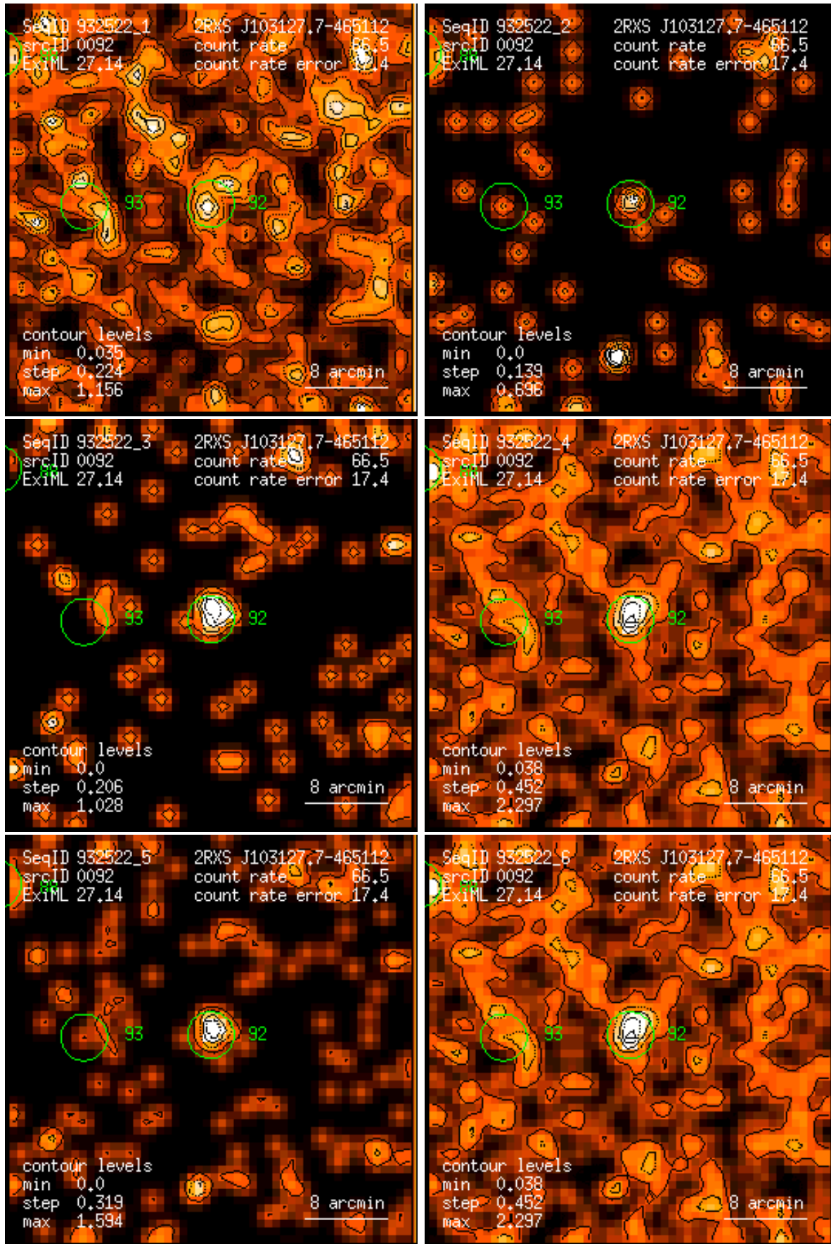
Figure 92: RASS 932522: detection 0092: band rate images, Gaussian filter: (1) PSPC channels 11 – 41, (2) 52 – 90, (3) 91 – 201, (4) 11 – 235, (5) 52 – 201, (6) 11 – 201. Broad band rates in counts/ks. Band rate contour levels in counts/ks/arcmin 2 .
