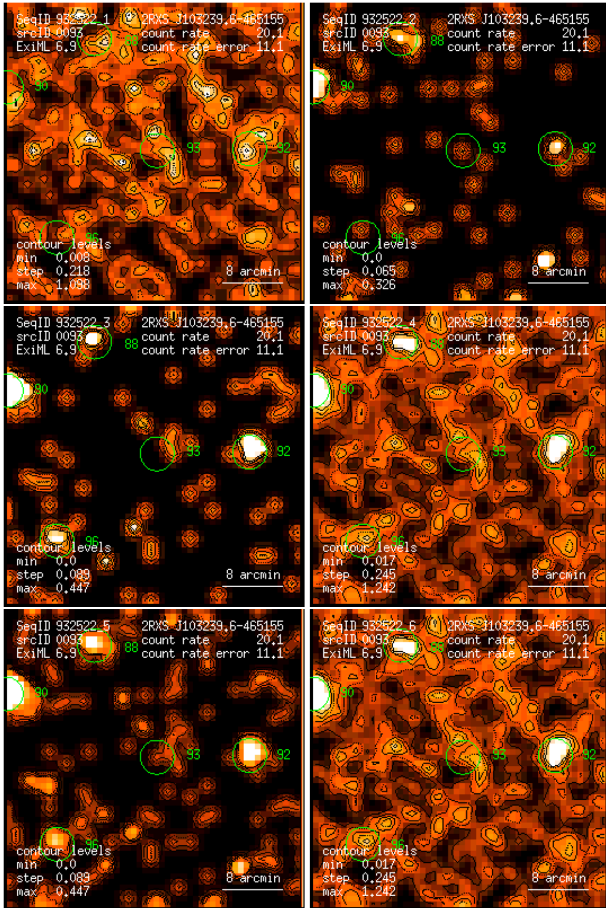
Figure 93: RASS 932522: detection 0093: band rate images, Gaussian filter: (1) PSPC channels 11 – 41, (2) 52 – 90, (3) 91 – 201, (4) 11 – 235, (5) 52 – 201, (6) 11 – 201. Broad band rates in counts/ks. Band rate contour levels in counts/ks/arcmin 2 .
