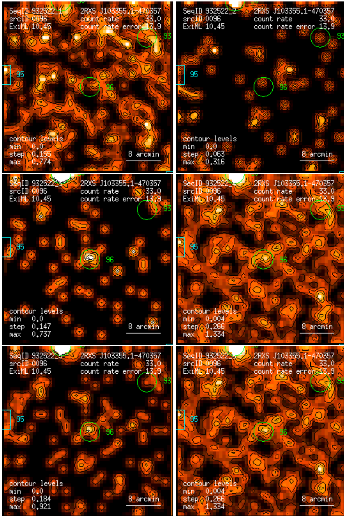
Figure 96: RASS 932522: detection 0096: band rate images, Gaussian filter: (1) PSPC channels 11 – 41, (2) 52 – 90, (3) 91 – 201, (4) 11 – 235, (5) 52 – 201, (6) 11 – 201. Broad band rates in counts/ks. Band rate contour levels in counts/ks/arcmin 2 .
