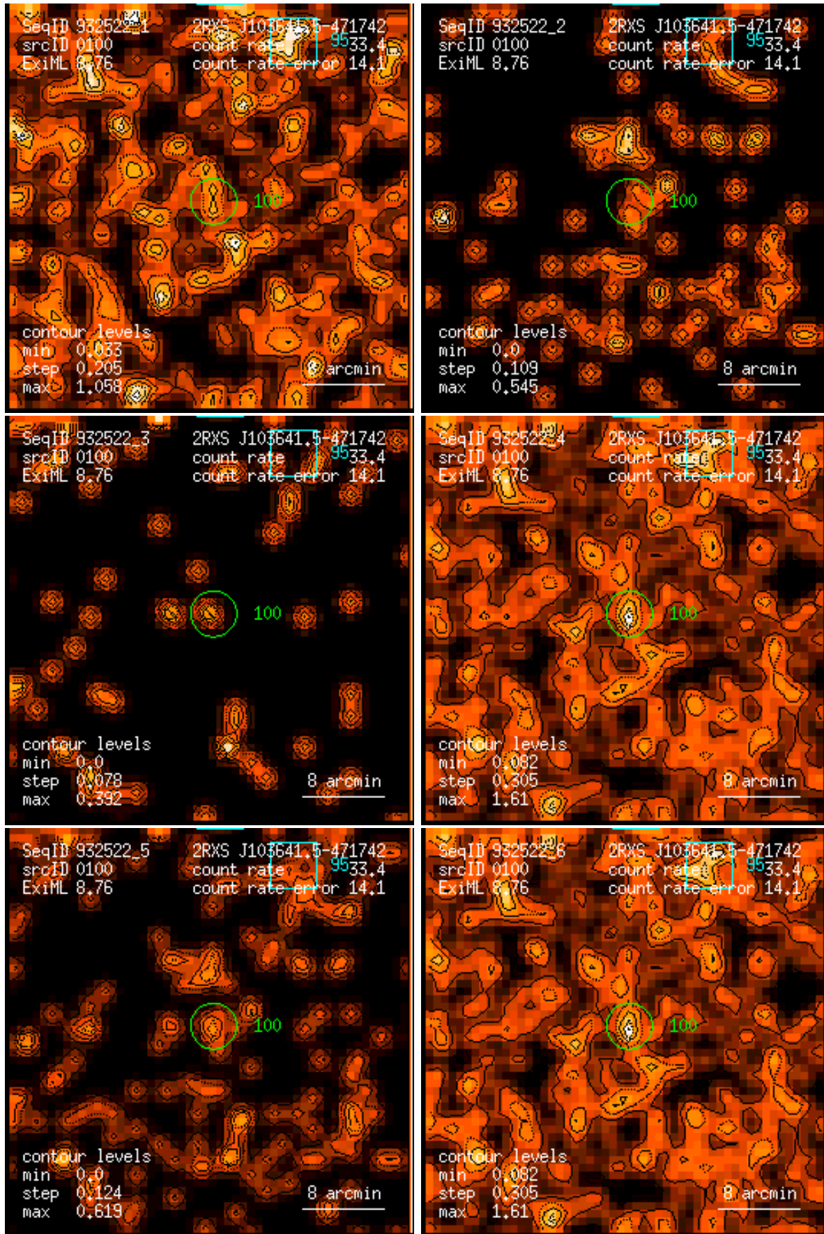
Figure 100: RASS 932522: detection 0100: band rate images, Gaussian filter: (1) PSPC channels 11 – 41, (2) 52 – 90, (3) 91 – 201, (4) 11 – 235, (5) 52 – 201, (6) 11 – 201. Broad band rates in counts/ks. Band rate contour levels in counts/ks/arcmin 2 .
