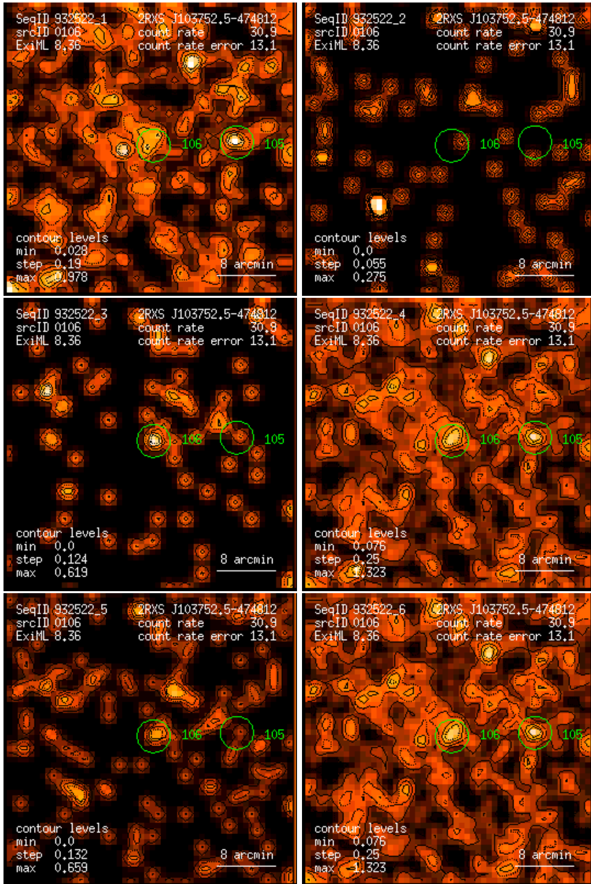
Figure 106: RASS 932522: detection 0106: band rate images, Gaussian filter: (1) PSPC channels 11 – 41, (2) 52 – 90, (3) 91 – 201, (4) 11 – 235, (5) 52 – 201, (6) 11 – 201. Broad band rates in counts/ks. Band rate contour levels in counts/ks/arcmin 2 .
