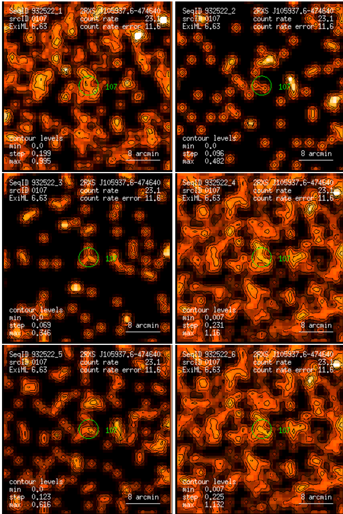
Figure 107: RASS 932522: detection 0107: band rate images, Gaussian filter: (1) PSPC channels 11 – 41, (2) 52 – 90, (3) 91 – 201, (4) 11 – 235, (5) 52 – 201, (6) 11 – 201. Broad band rates in counts/ks. Band rate contour levels in counts/ks/arcmin 2 .
