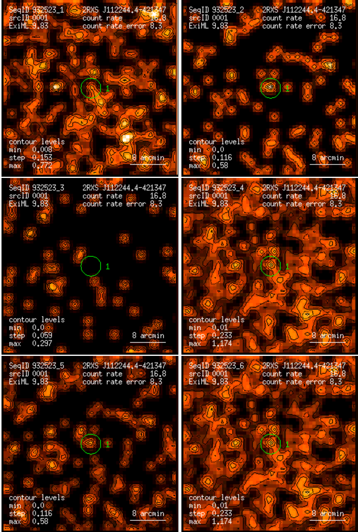
Figure 1: RASS 932523: detection 0001: band rate images, Gaussian filter: (1) PSPC channels 11 – 41, (2) 52 – 90, (3) 91 – 201, (4) 11 – 235, (5) 52 – 201, (6) 11 – 201. Broad band rates in counts/ks. Band rate contour levels in counts/ks/arcmin 2 .
